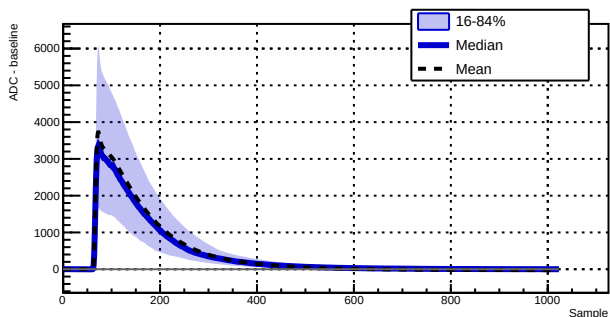
Run 039522 - Channel 1070 - 1624 waveforms
