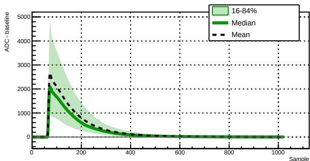
Run 039522 - Channel 1060 - 9267 waveforms
