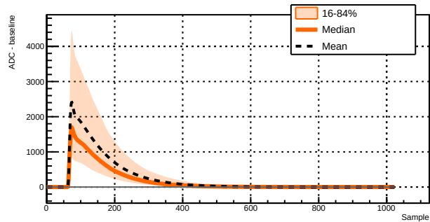
Run 039522 - Channel 1011 - 17210 waveforms
