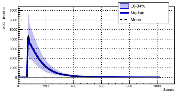
Run 039522 - Channel 1030 - 4438 waveforms
