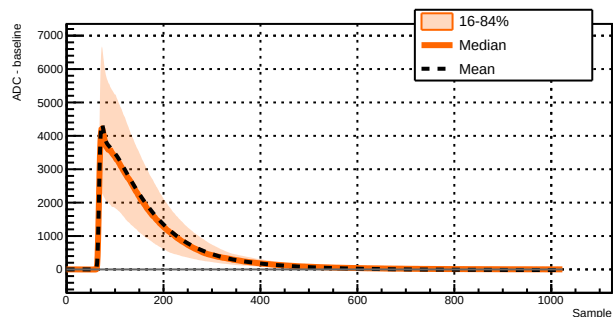
Run 039522 - Channel 1071 - 1884 waveforms
