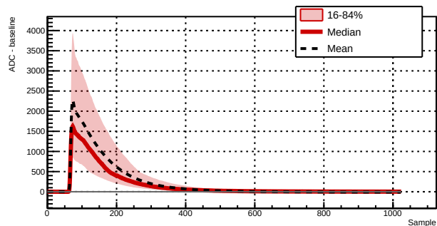
Run 039522 - Channel 1021 - 3081 waveforms
