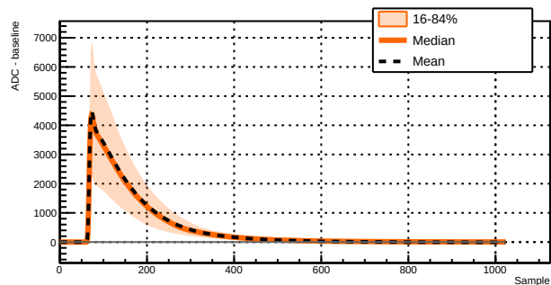
Run 039522 - Channel 1031 - 6324 waveforms
