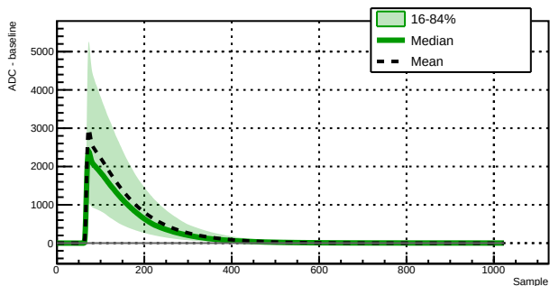
Run 039522 - Channel 1020 - 13644 waveforms
