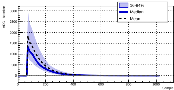
Run 039522 - Channel 1010 - 6651 waveforms
