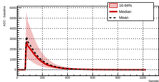
Run 039522 - Channel 1061 - 8107 waveforms
