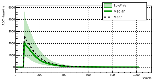
Run 039523 - Channel 1060 - 9164 waveforms
