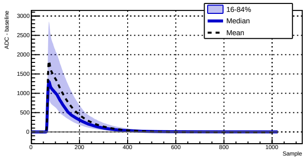
Run 039523 - Channel 1010 - 6546 waveforms
