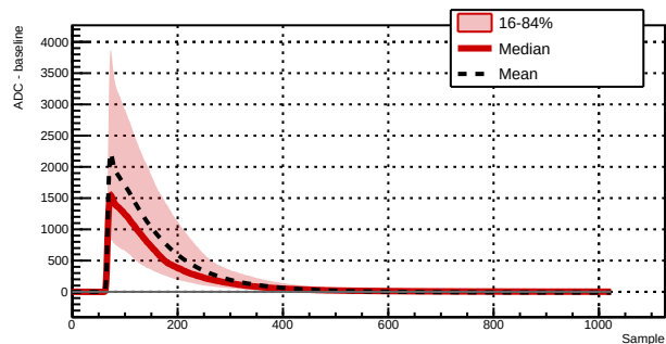
Run 039523 - Channel 1021 - 3000 waveforms
