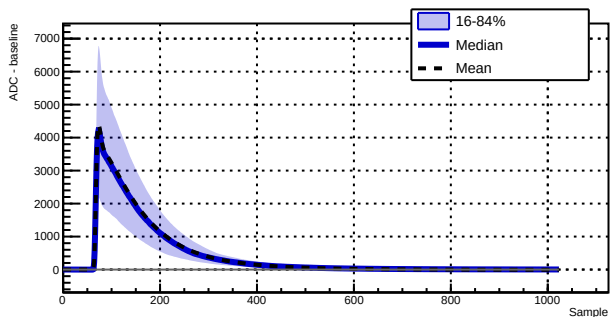
Run 039523 - Channel 1030 - 4237 waveforms
