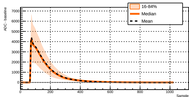
Run 039523 - Channel 1071 - 1923 waveforms
