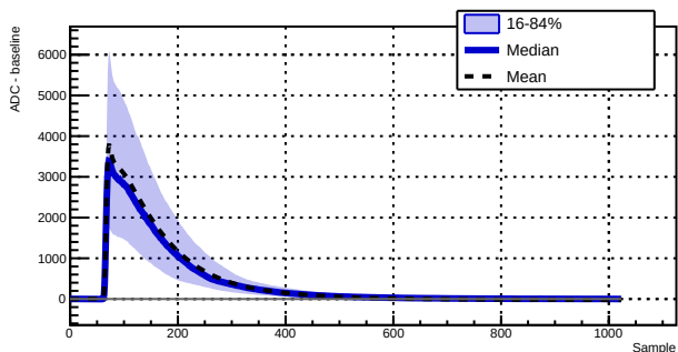
Run 039523 - Channel 1070 - 1533 waveforms
