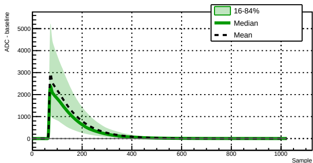
Run 039523 - Channel 1020 - 13442 waveforms
