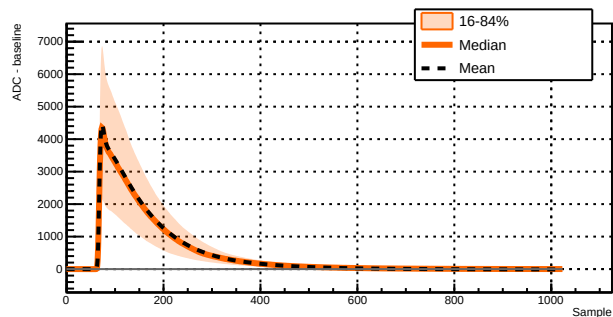
Run 039523 - Channel 1031 - 5655 waveforms
