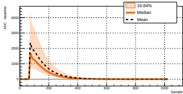
Run 039523 - Channel 1011 - 16715 waveforms
