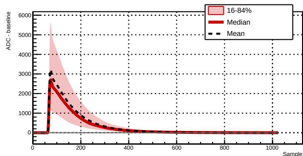
Run 039523 - Channel 1061 - 7990 waveforms
