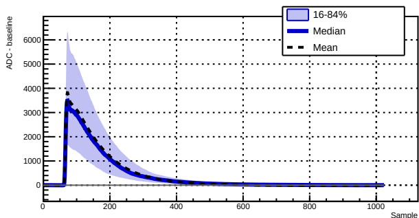
Run 039525 - Channel 1070 - 1637 waveforms
