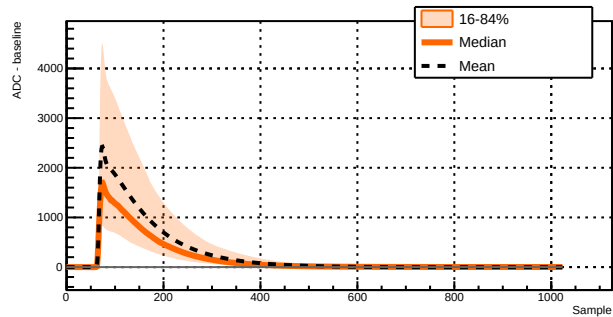
Run 039525 - Channel 1011 - 17236 waveforms
