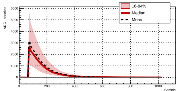
Run 039525 - Channel 1061 - 7903 waveforms
