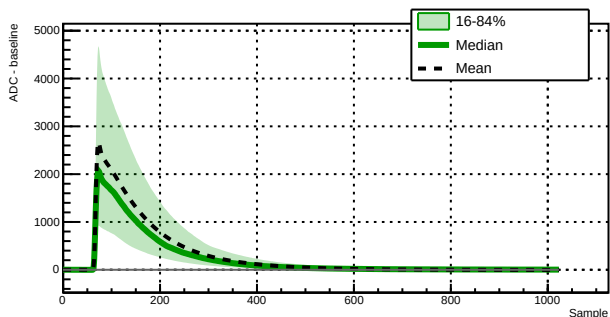
Run 039525 - Channel 1060 - 8950 waveforms
