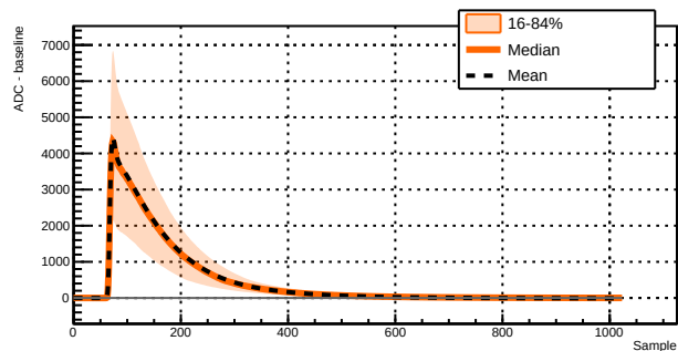
Run 039525 - Channel 1031 - 5703 waveforms
