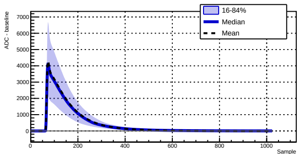
Run 039525 - Channel 1030 - 4189 waveforms
