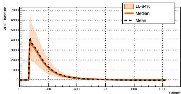
Run 039525 - Channel 1071 - 1929 waveforms
