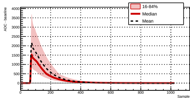
Run 039525 - Channel 1021 - 2838 waveforms
