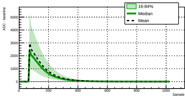
Run 039525 - Channel 1020 - 13338 waveforms
