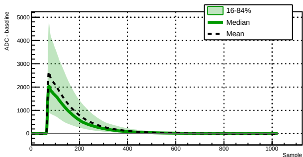
Run 039526 - Channel 1060 - 9011 waveforms
