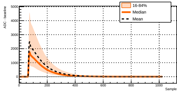
Run 039526 - Channel 1011 - 17850 waveforms
