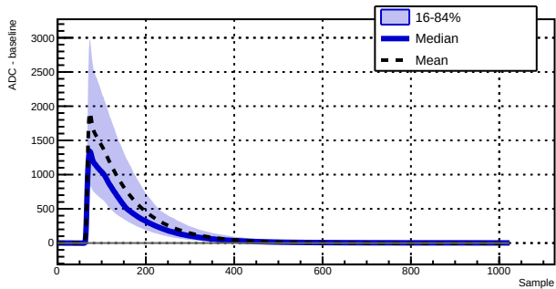
Run 039526 - Channel 1010 - 6738 waveforms
