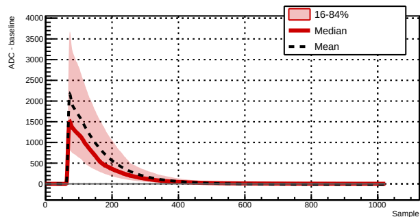
Run 039526 - Channel 1021 - 2796 waveforms
