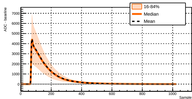
Run 039526 - Channel 1031 - 5667 waveforms
