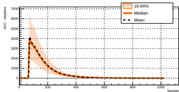
Run 039526 - Channel 1071 - 1988 waveforms
