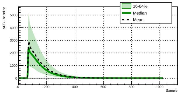
Run 039526 - Channel 1020 - 13364 waveforms
