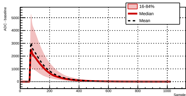
Run 039526 - Channel 1061 - 7575 waveforms
