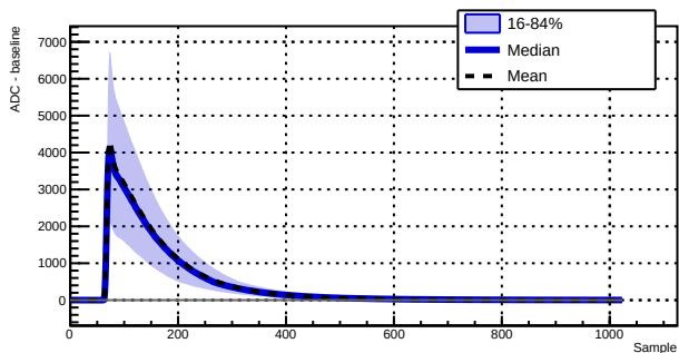
Run 039526 - Channel 1030 - 4143 waveforms
