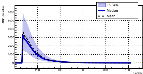
Run 039526 - Channel 1070 - 1610 waveforms
