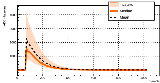
Run 039527 - Channel 1011 - 15808 waveforms
