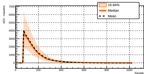
Run 039527 - Channel 1071 - 1581 waveforms
