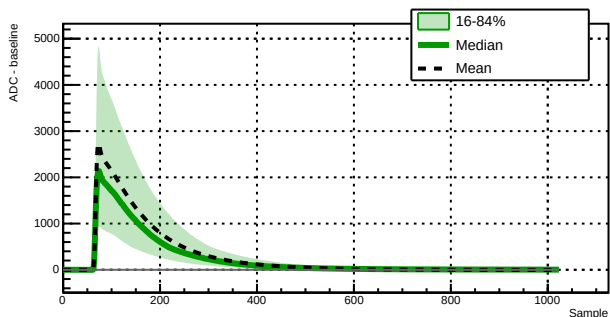
Run 039527 - Channel 1060 - 9204 waveforms
