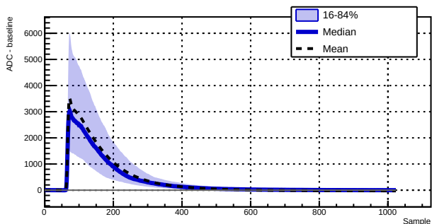
Run 039527 - Channel 1070 - 1275 waveforms
