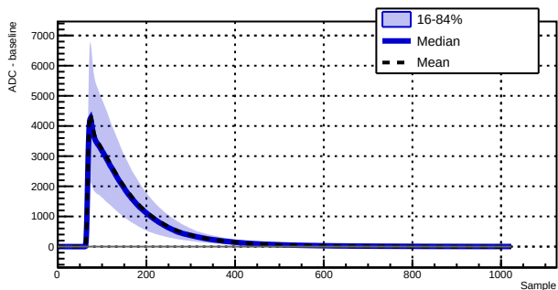
Run 039527 - Channel 1030 - 4287 waveforms
