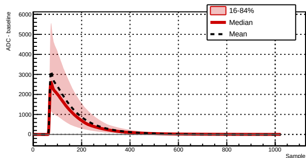
Run 039527 - Channel 1061 - 7466 waveforms
