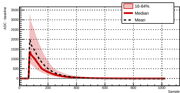
Run 039527 - Channel 1021 - 2367 waveforms
