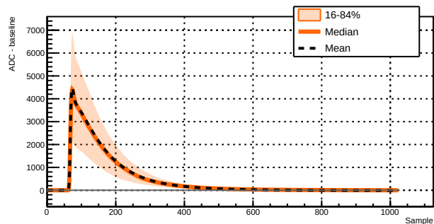
Run 039527 - Channel 1031 - 5055 waveforms
