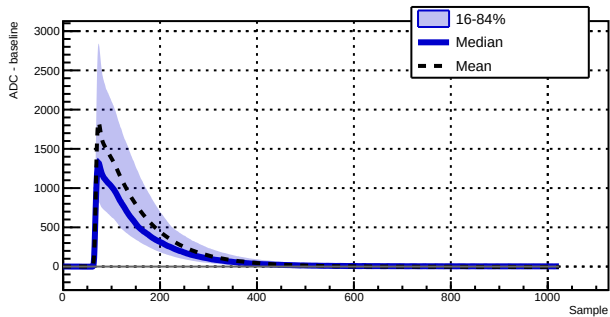
Run 039527 - Channel 1010 - 6813 waveforms
