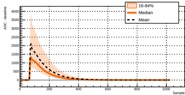
Run 039528 - Channel 1011 - 13777 waveforms
