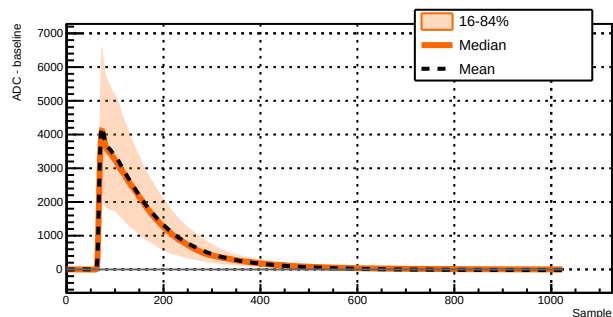
Run 039528 - Channel 1071 - 1794 waveforms
