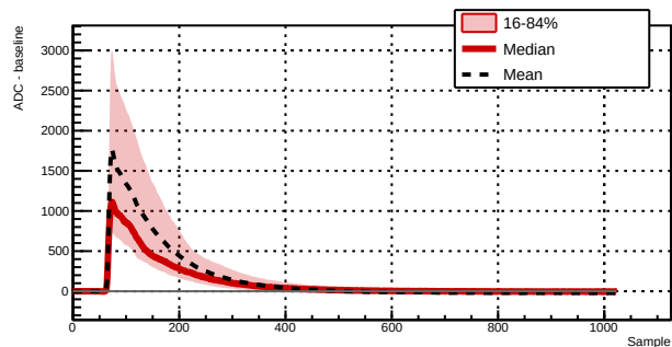
Run 039528 - Channel 1021 - 1872 waveforms
