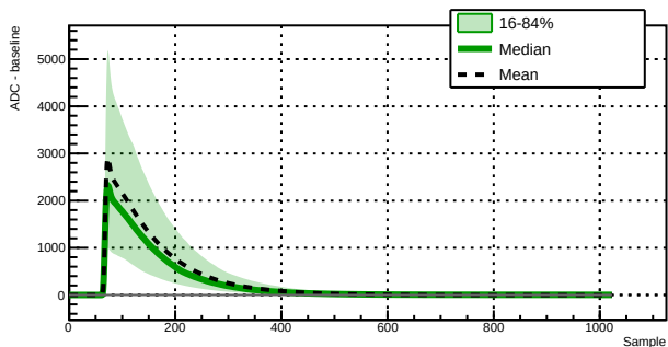
Run 039528 - Channel 1020 - 12507 waveforms
