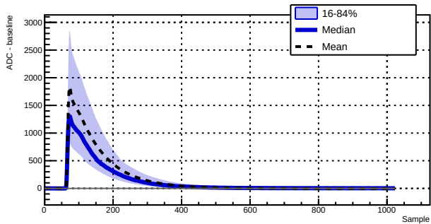
Run 039528 - Channel 1010 - 6783 waveforms
