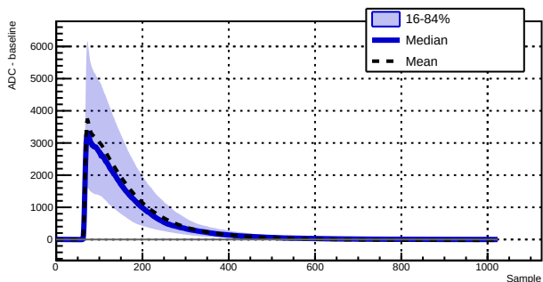
Run 039528 - Channel 1070 - 1650 waveforms
