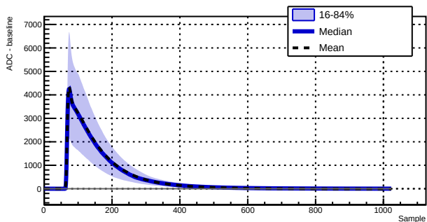
Run 039528 - Channel 1030 - 4108 waveforms
