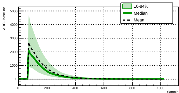
Run 039528 - Channel 1060 - 8894 waveforms
