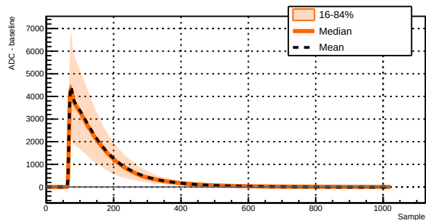
Run 039528 - Channel 1031 - 5025 waveforms
