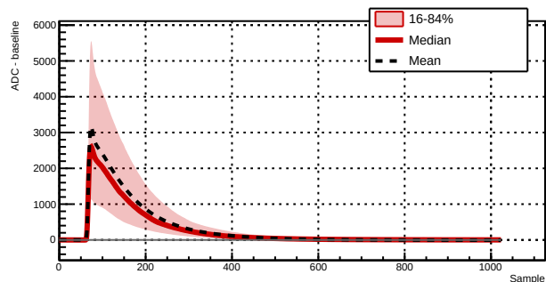
Run 039528 - Channel 1061 - 7285 waveforms
