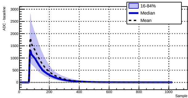
Run 039529 - Channel 1010 - 6690 waveforms
