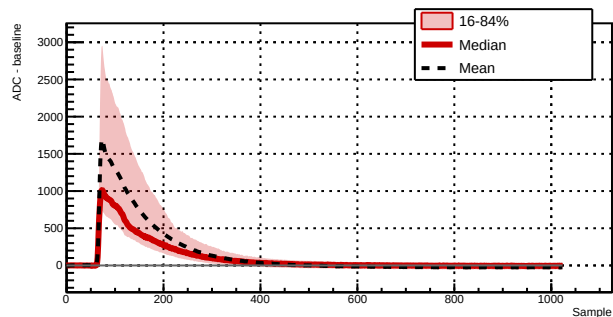
Run 039529 - Channel 1021 - 1528 waveforms
