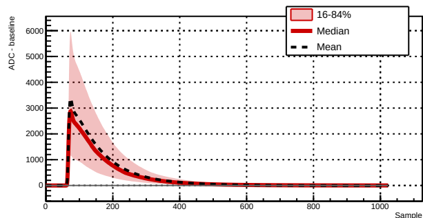
Run 039529 - Channel 1061 - 7413 waveforms
