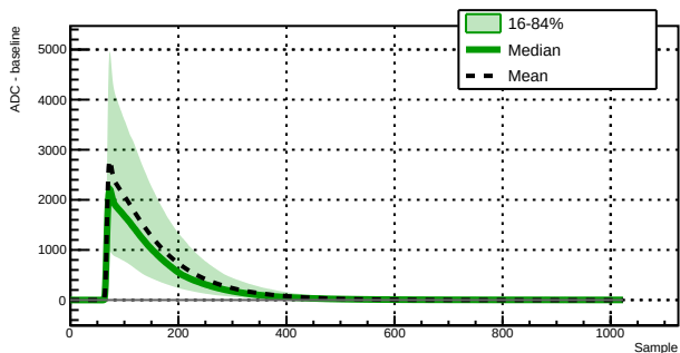
Run 039529 - Channel 1020 - 12038 waveforms
