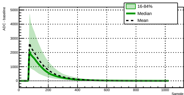
Run 039529 - Channel 1060 - 9044 waveforms
