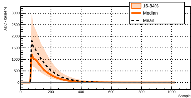
Run 039529 - Channel 1011 - 11165 waveforms
