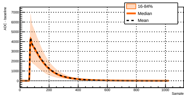
Run 039529 - Channel 1031 - 4662 waveforms
