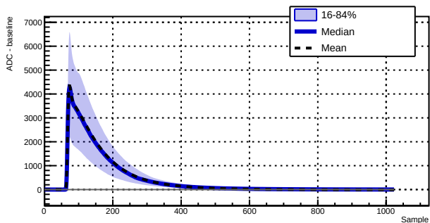
Run 039529 - Channel 1030 - 3927 waveforms
