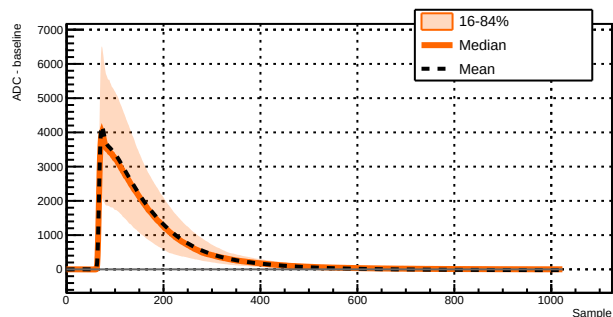
Run 039529 - Channel 1071 - 1814 waveforms
