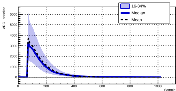
Run 039529 - Channel 1070 - 1605 waveforms
