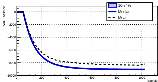
Run 040931 - Channel 1030 - 219 waveforms
