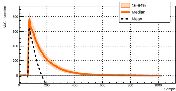
Run 040931 - Channel 1011 - 382 waveforms
