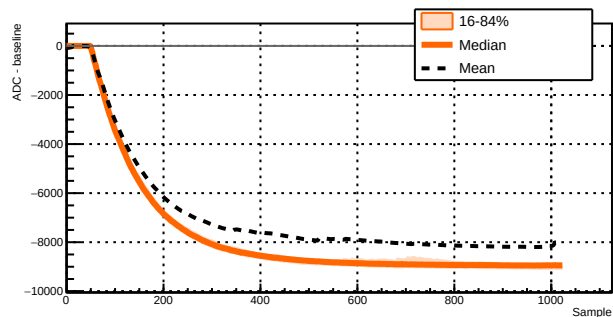
Run 040931 - Channel 1031 - 193 waveforms
