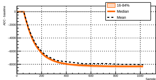
Run 040931 - Channel 1071 - 206 waveforms
