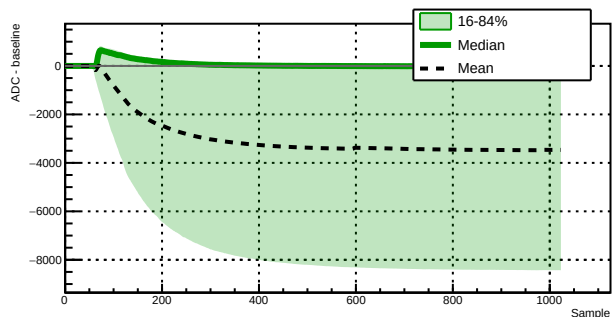
Run 040931 - Channel 1060 - 274 waveforms
