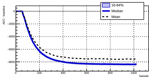
Run 040931 - Channel 1070 - 199 waveforms
