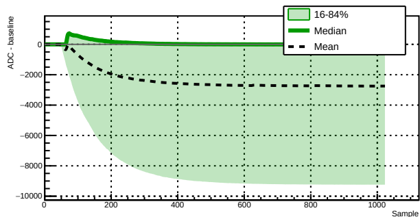
Run 040931 - Channel 1020 - 232 waveforms
