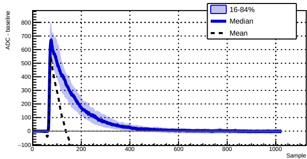
Run 040931 - Channel 1010 - 200 waveforms
