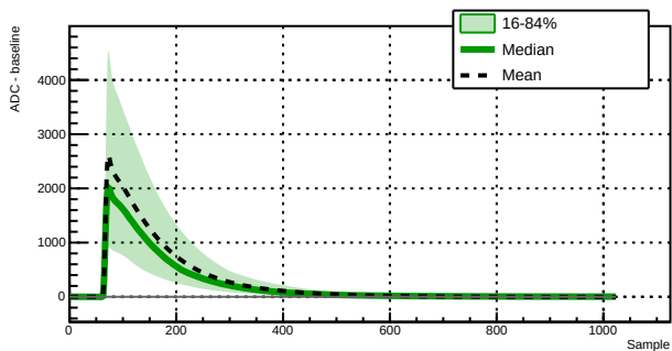
Run 043380 - Channel 1060 - 9657 waveforms
