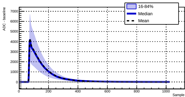
Run 043380 - Channel 1030 - 4433 waveforms
