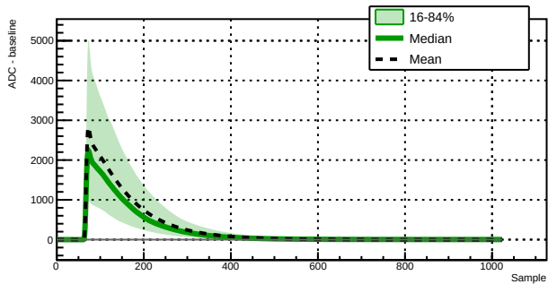
Run 043380 - Channel 1020 - 12730 waveforms
