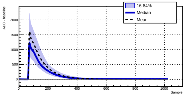
Run 043380 - Channel 1010 - 5887 waveforms
