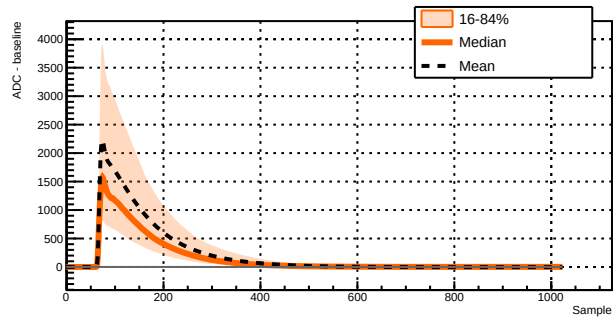
Run 043380 - Channel 1011 - 15454 waveforms
