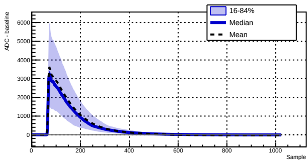
Run 043380 - Channel 1070 - 1606 waveforms
