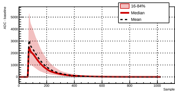
Run 043380 - Channel 1061 - 7726 waveforms
