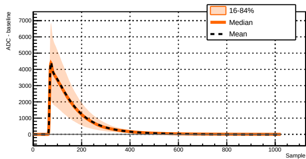
Run 043380 - Channel 1031 - 5019 waveforms
