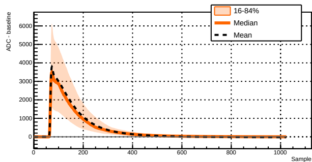
Run 043380 - Channel 1071 - 1226 waveforms
