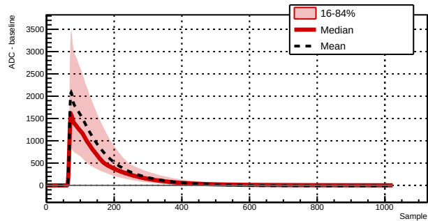
Run 043380 - Channel 1021 - 5595 waveforms
