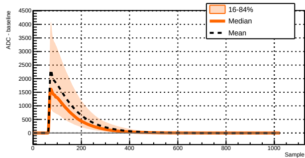
Run 043383 - Channel 1011 - 15760 waveforms
