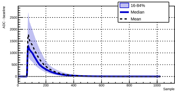
Run 043383 - Channel 1010 - 6955 waveforms
