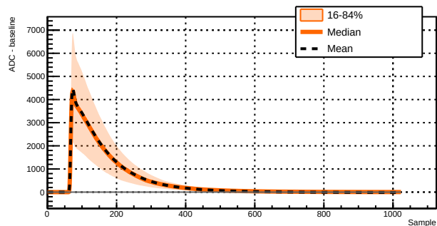
Run 043383 - Channel 1031 - 4323 waveforms
