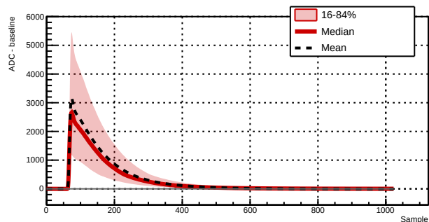
Run 043383 - Channel 1061 - 7953 waveforms
