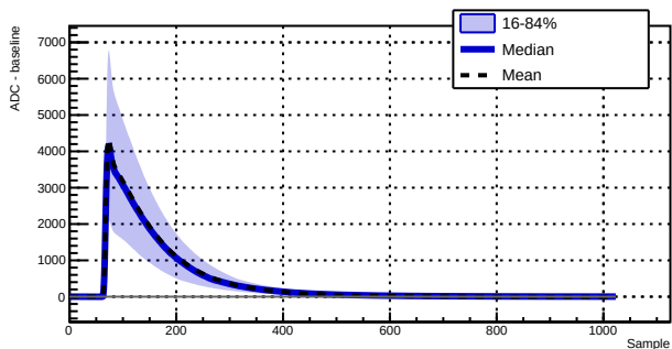
Run 043383 - Channel 1030 - 4573 waveforms
