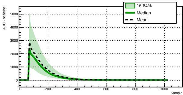
Run 043383 - Channel 1020 - 13069 waveforms
