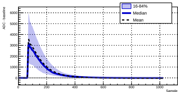
Run 043383 - Channel 1070 - 1464 waveforms
