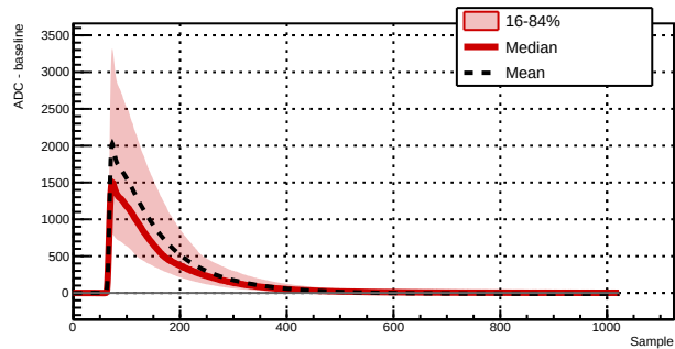
Run 043383 - Channel 1021 - 4435 waveforms
