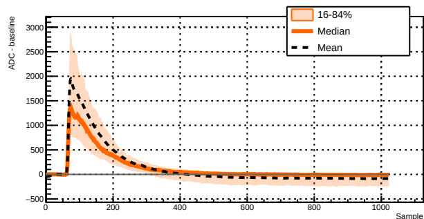
Run 043383 - Channel 1071 - 199 waveforms
