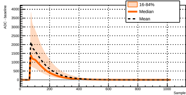
Run 043386 - Channel 1011 - 15338 waveforms
