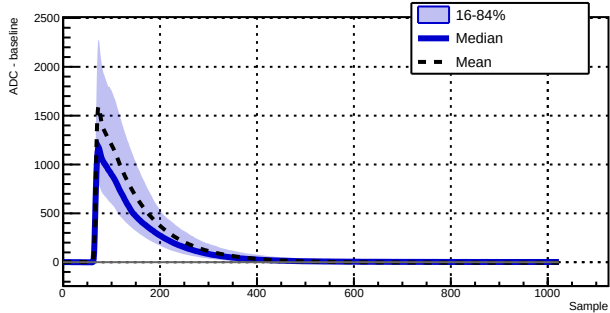
Run 043386 - Channel 1010 - 6243 waveforms
