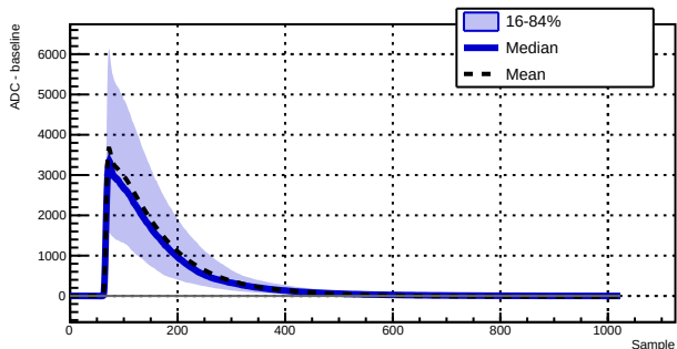
Run 043386 - Channel 1070 - 1786 waveforms
