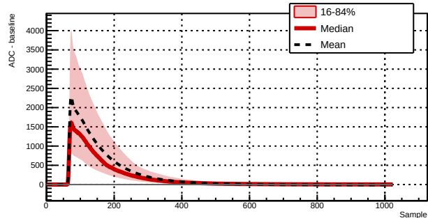
Run 043386 - Channel 1021 - 3895 waveforms
