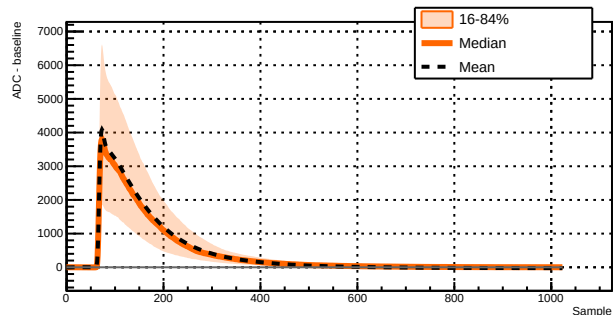
Run 043386 - Channel 1071 - 1673 waveforms
