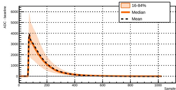
Run 043386 - Channel 1031 - 2173 waveforms
