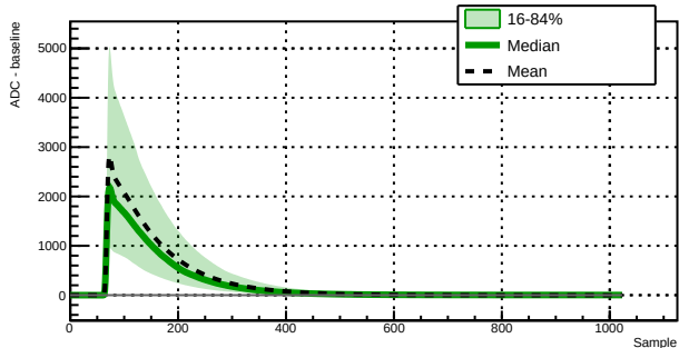
Run 043386 - Channel 1020 - 13150 waveforms
