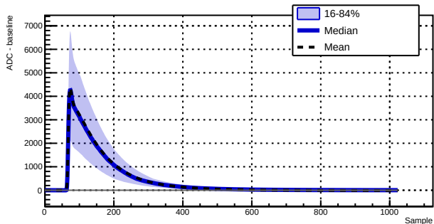
Run 043386 - Channel 1030 - 4270 waveforms
