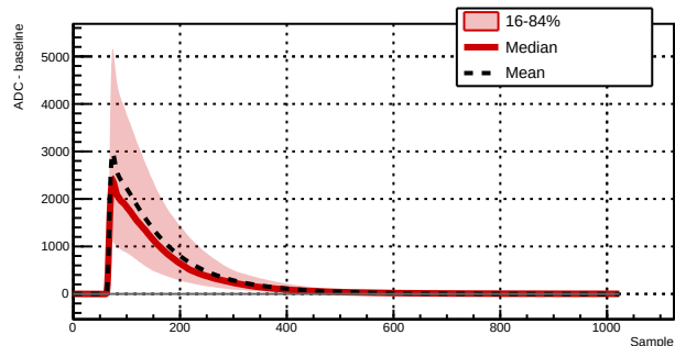
Run 043386 - Channel 1061 - 7128 waveforms
