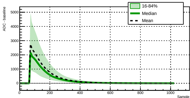
Run 043386 - Channel 1060 - 9414 waveforms
