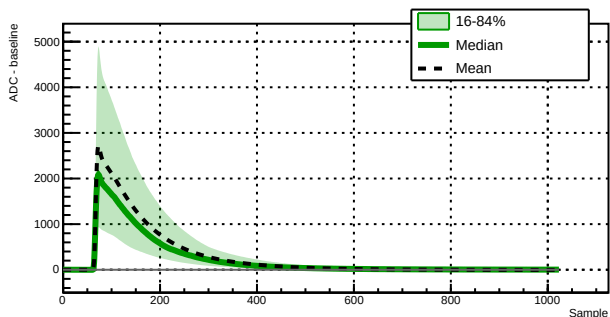
Run 043387 - Channel 1060 - 9467 waveforms
