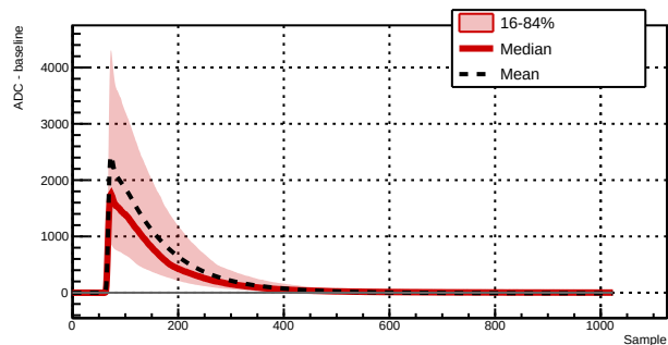
Run 043387 - Channel 1021 - 4073 waveforms
