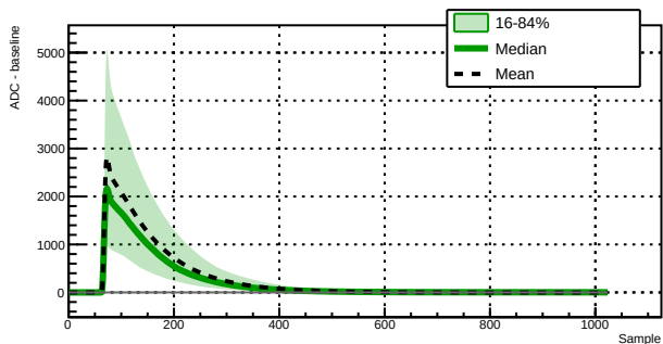
Run 043387 - Channel 1020 - 13420 waveforms
