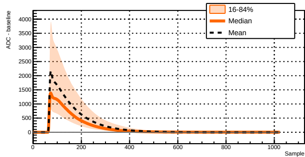
Run 043387 - Channel 1011 - 15288 waveforms
