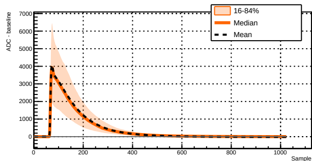
Run 043387 - Channel 1031 - 2544 waveforms
