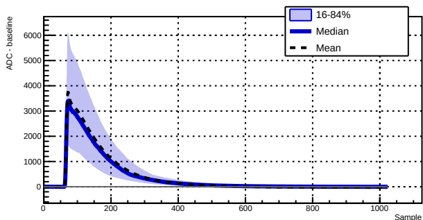
Run 043387 - Channel 1070 - 1786 waveforms
