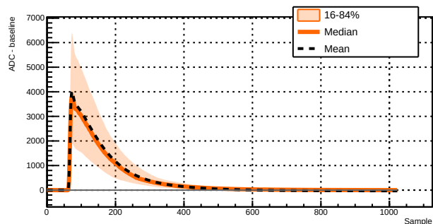
Run 043387 - Channel 1071 - 1645 waveforms
