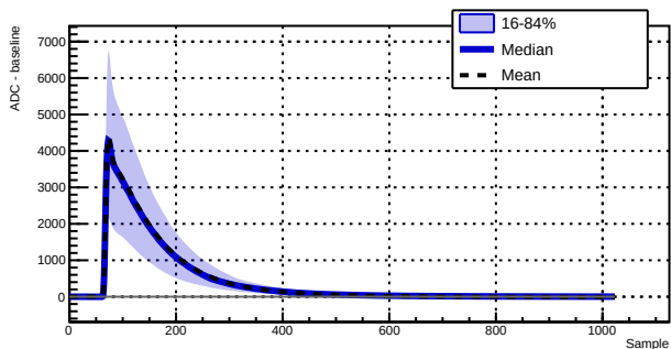
Run 043387 - Channel 1030 - 4297 waveforms
