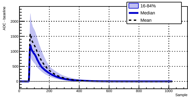
Run 043387 - Channel 1010 - 6165 waveforms
