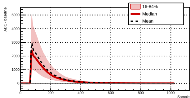
Run 043387 - Channel 1061 - 7152 waveforms
