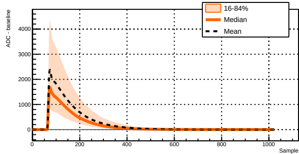
Run 043389 - Channel 1011 - 17128 waveforms
