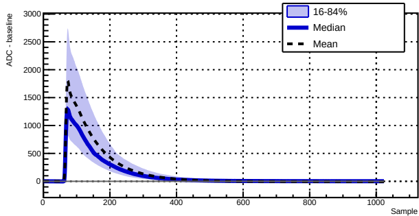
Run 043389 - Channel 1010 - 6659 waveforms
