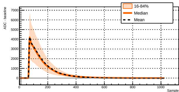
Run 043389 - Channel 1031 - 2798 waveforms
