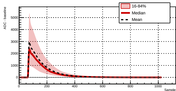
Run 043389 - Channel 1061 - 6143 waveforms
