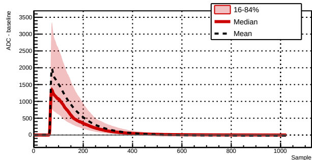
Run 043389 - Channel 1021 - 2265 waveforms
