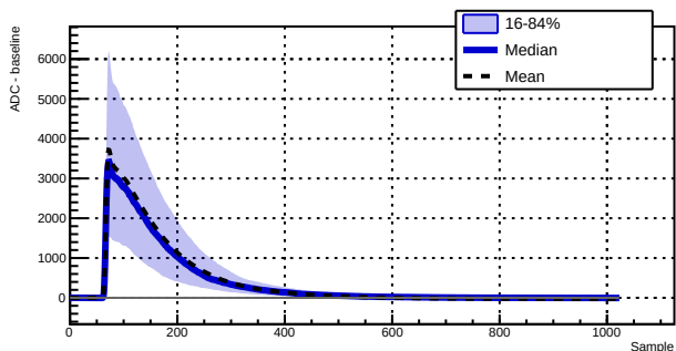
Run 043389 - Channel 1070 - 1482 waveforms
