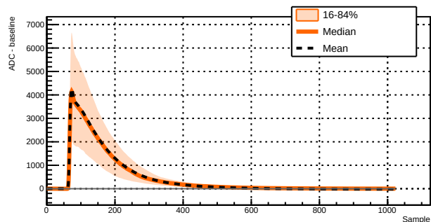
Run 043389 - Channel 1071 - 1672 waveforms
