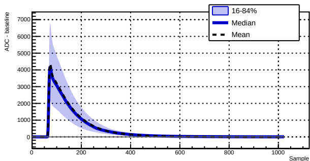
Run 043389 - Channel 1030 - 4072 waveforms
