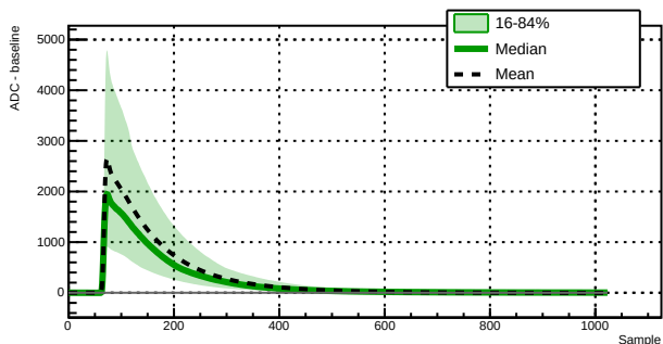
Run 043389 - Channel 1060 - 9660 waveforms
