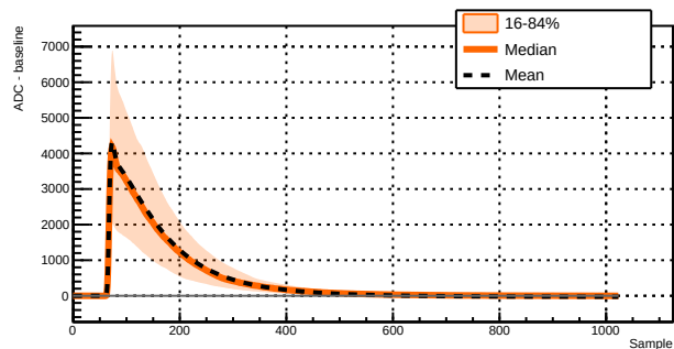
Run 043390 - Channel 1031 - 2660 waveforms
