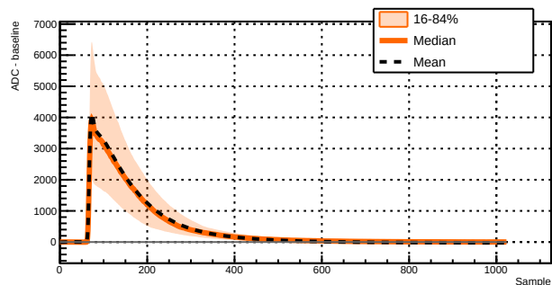
Run 043390 - Channel 1071 - 1614 waveforms
