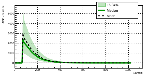
Run 043390 - Channel 1020 - 14124 waveforms
