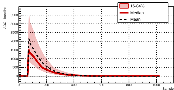
Run 043390 - Channel 1021 - 2513 waveforms
