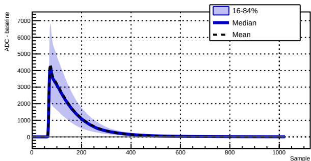
Run 043390 - Channel 1030 - 4167 waveforms
