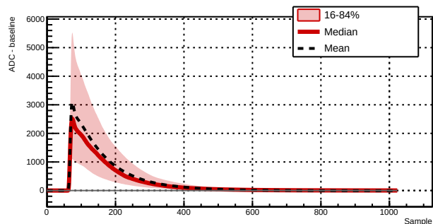
Run 043390 - Channel 1061 - 6185 waveforms
