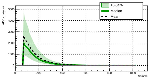
Run 043390 - Channel 1060 - 9686 waveforms
