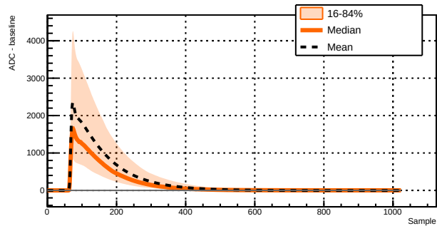
Run 043390 - Channel 1011 - 16962 waveforms
