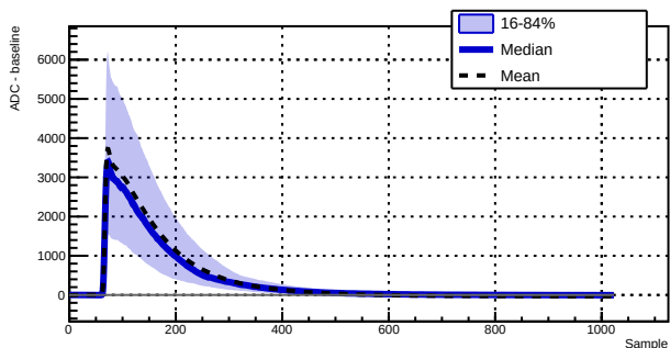
Run 043390 - Channel 1070 - 1470 waveforms
