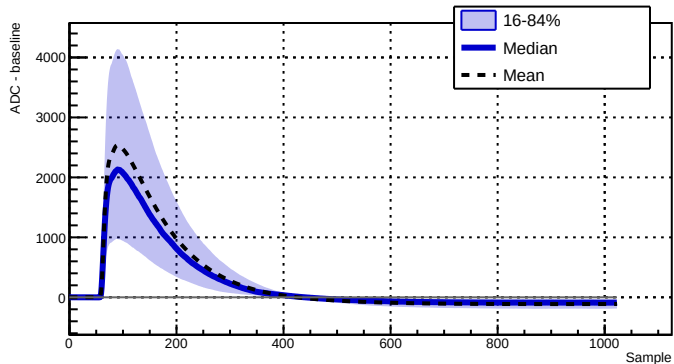
Run 039500 - Channel 2050 - 2274 waveforms
