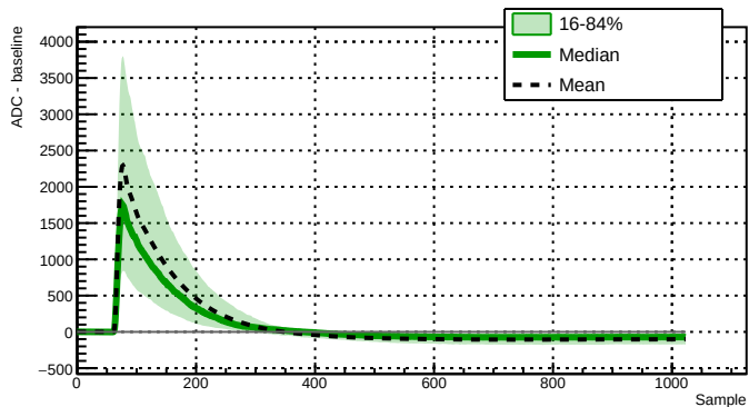
Run 039500 - Channel 2060 - 569 waveforms
