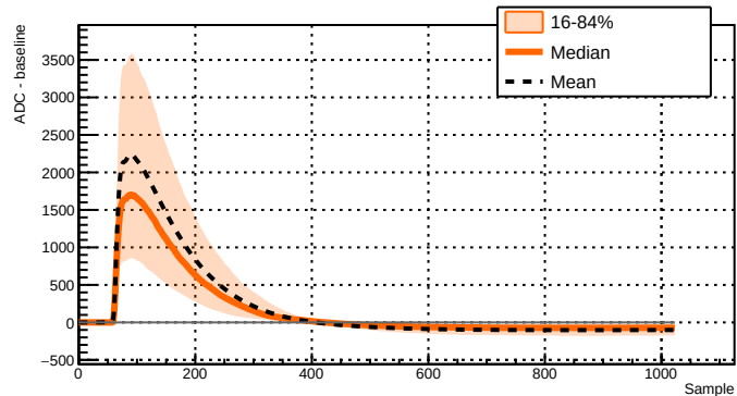
Run 039500 - Channel 2051 - 1709 waveforms
