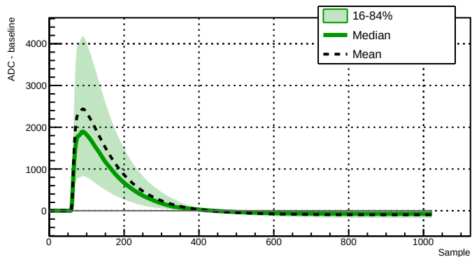
Run 039500 - Channel 2080 - 6944 waveforms
