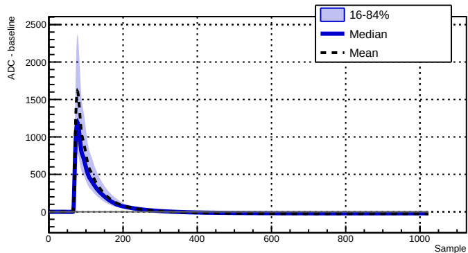
Run 039500 - Channel 2070 - 2673 waveforms
