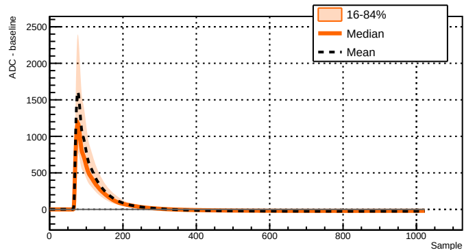
Run 039500 - Channel 2071 - 2968 waveforms
