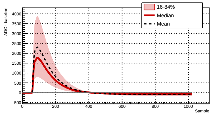
Run 039500 - Channel 2081 - 8788 waveforms
