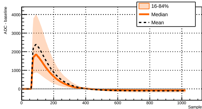
Run 039501 - Channel 2051 - 1831 waveforms
