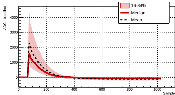
Run 039501 - Channel 2061 - 420 waveforms
