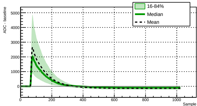
Run 039501 - Channel 2060 - 551 waveforms
