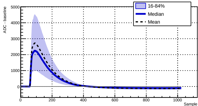
Run 039501 - Channel 2050 - 2362 waveforms
