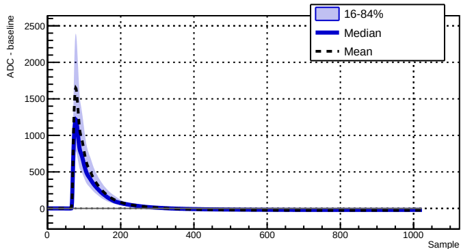
Run 039501 - Channel 2070 - 2765 waveforms
