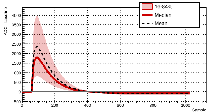
Run 039501 - Channel 2081 - 9041 waveforms
