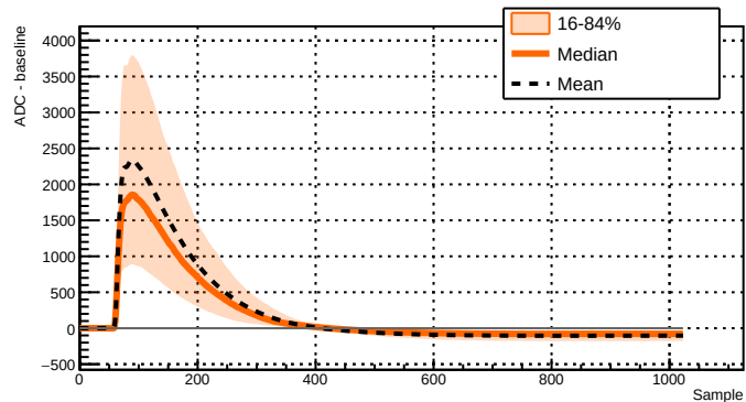
Run 039502 - Channel 2051 - 1893 waveforms
