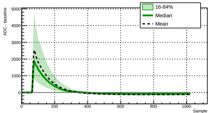
Run 039502 - Channel 2060 - 606 waveforms
