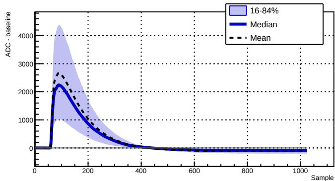
Run 039502 - Channel 2050 - 2602 waveforms
