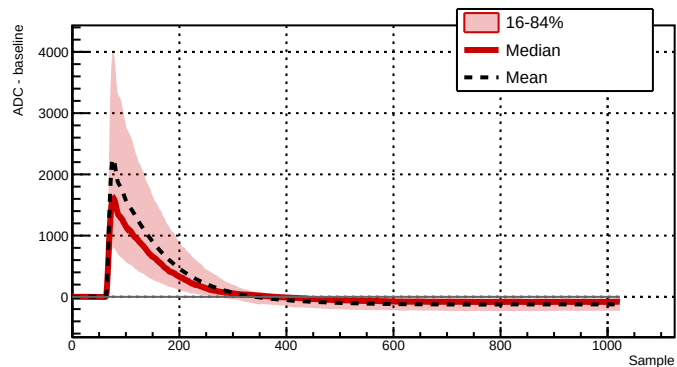
Run 039502 - Channel 2061 - 392 waveforms
