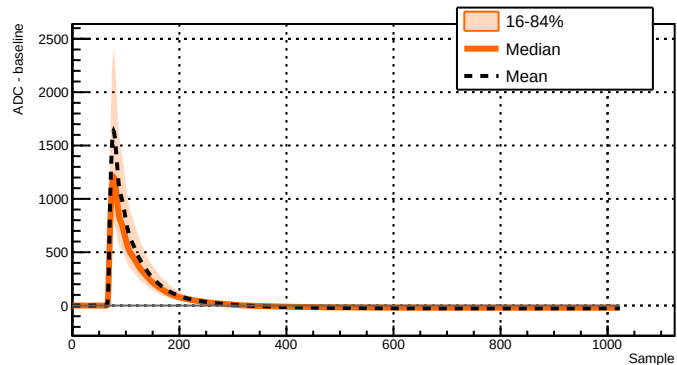
Run 039502 - Channel 2071 - 3027 waveforms
