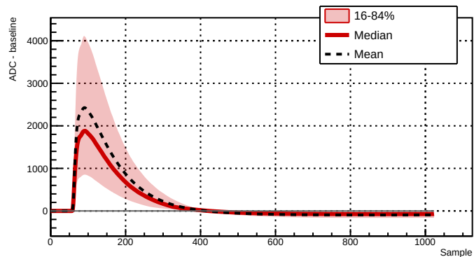
Run 039502 - Channel 2081 - 9337 waveforms
