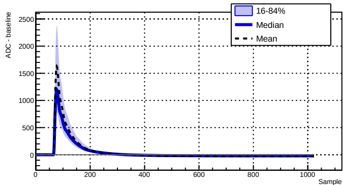
Run 039502 - Channel 2070 - 2777 waveforms
