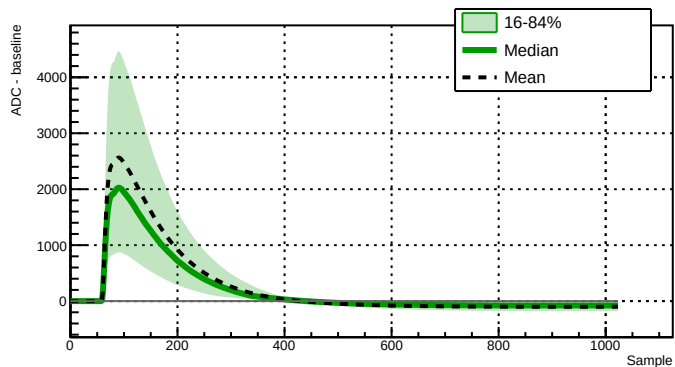
Run 039502 - Channel 2080 - 7515 waveforms
