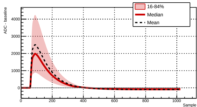
Run 039503 - Channel 2081 - 9889 waveforms
