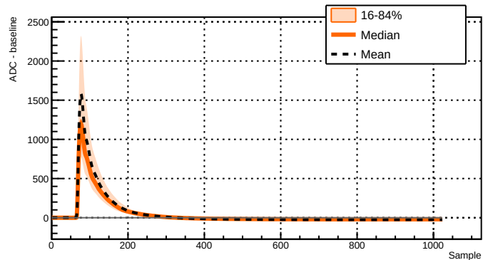
Run 039503 - Channel 2071 - 3111 waveforms
