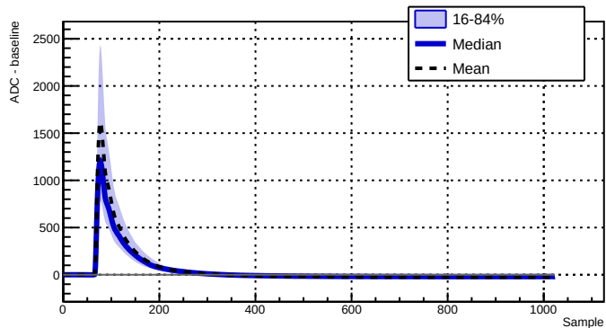
Run 039503 - Channel 2070 - 2935 waveforms
