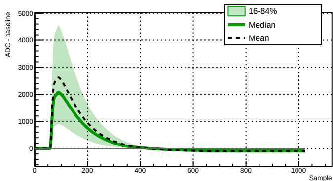
Run 039503 - Channel 2080 - 7944 waveforms
