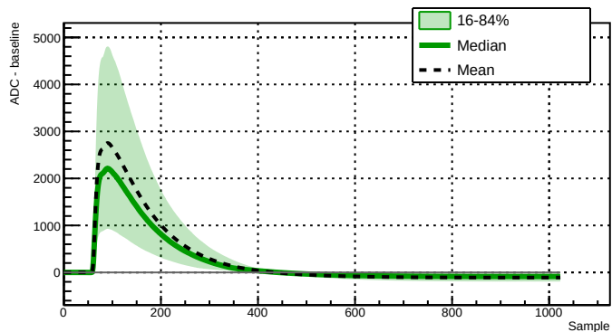
Run 039504 - Channel 2080 - 8106 waveforms
