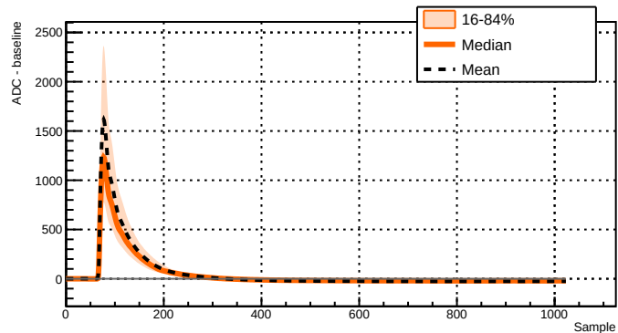
Run 039504 - Channel 2071 - 3063 waveforms
