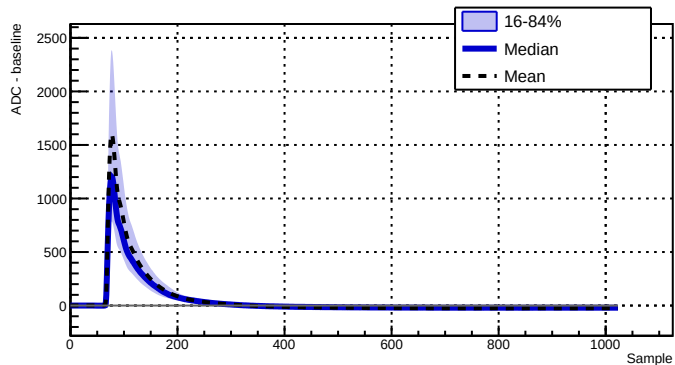
Run 039504 - Channel 2070 - 2911 waveforms
