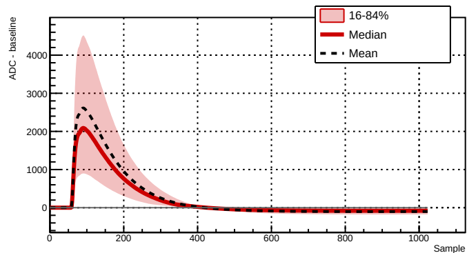
Run 039504 - Channel 2081 - 10322 waveforms
