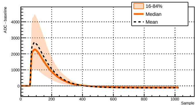
Run 039506 - Channel 2051 - 2447 waveforms
