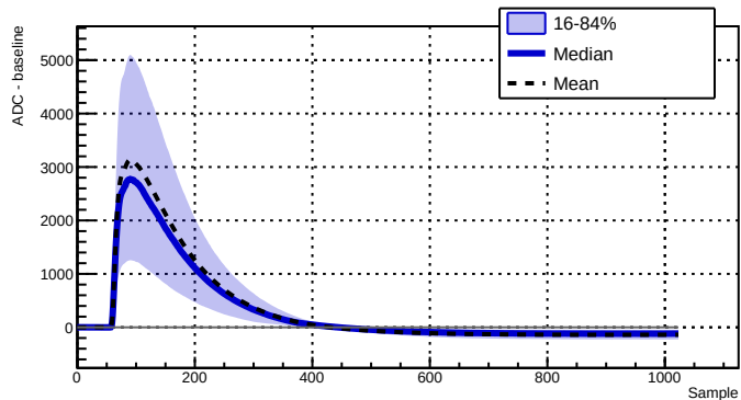
Run 039506 - Channel 2050 - 3349 waveforms
