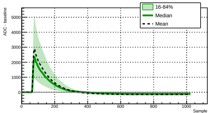
Run 039506 - Channel 2060 - 784 waveforms
