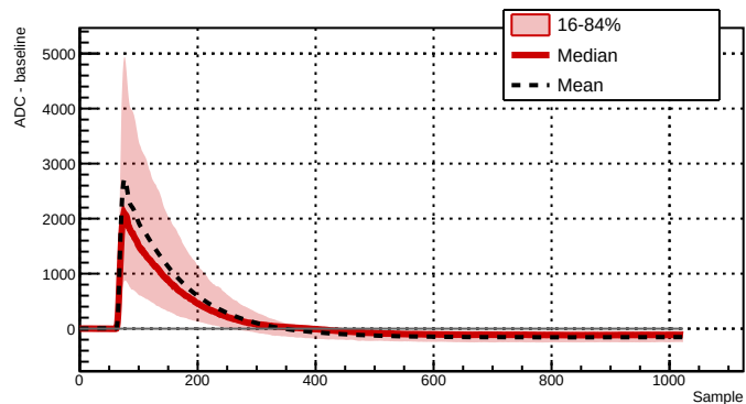
Run 039506 - Channel 2061 - 499 waveforms
