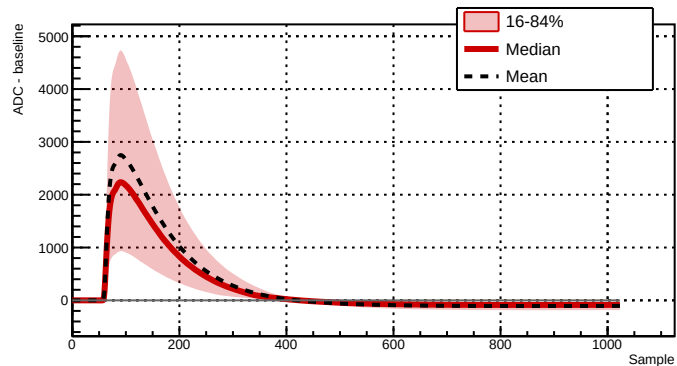
Run 039506 - Channel 2081 - 10921 waveforms
