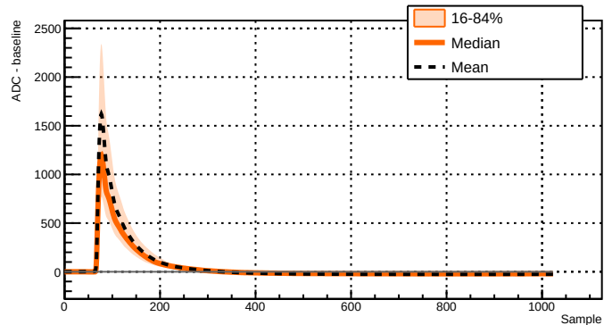
Run 039506 - Channel 2071 - 3204 waveforms
