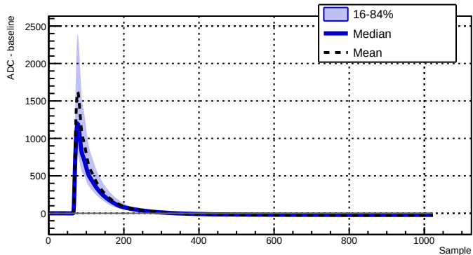
Run 039506 - Channel 2070 - 3062 waveforms
