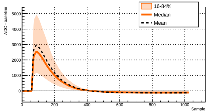
Run 039507 - Channel 2051 - 2705 waveforms
