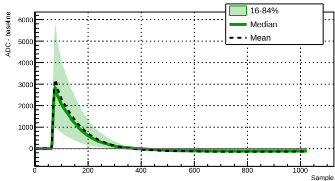
Run 039507 - Channel 2060 - 795 waveforms
