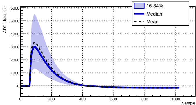
Run 039507 - Channel 2050 - 3652 waveforms
