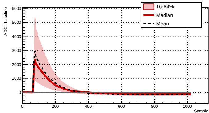
Run 039507 - Channel 2061 - 493 waveforms
