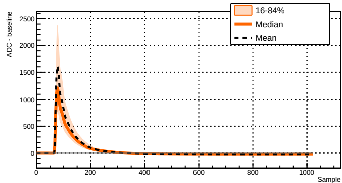
Run 039507 - Channel 2071 - 3148 waveforms
