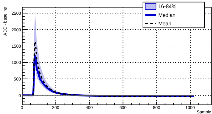
Run 039507 - Channel 2070 - 3003 waveforms
