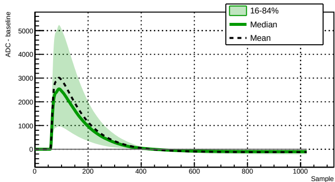
Run 039507 - Channel 2080 - 9268 waveforms
