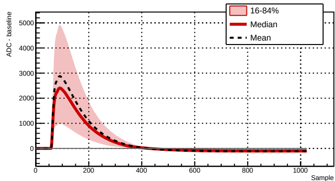
Run 039507 - Channel 2081 - 11559 waveforms
