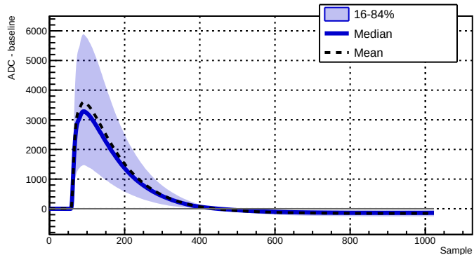
Run 039508 - Channel 2050 - 3998 waveforms
