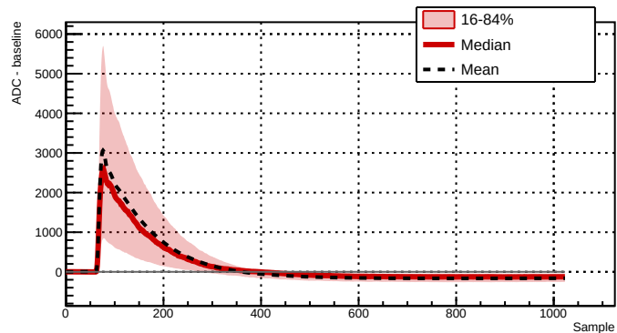
Run 039508 - Channel 2061 - 545 waveforms
