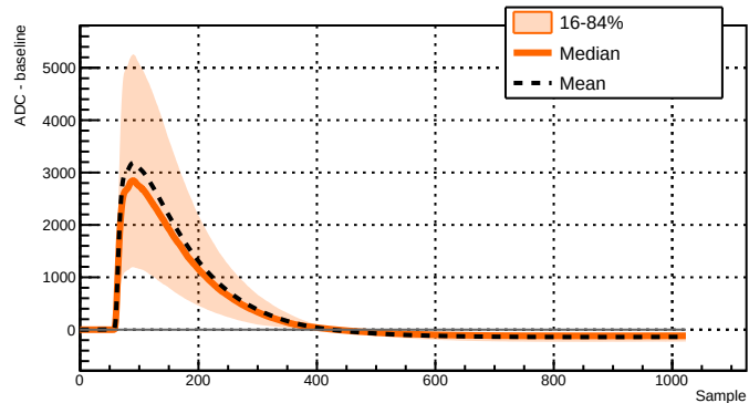
Run 039508 - Channel 2051 - 3003 waveforms
