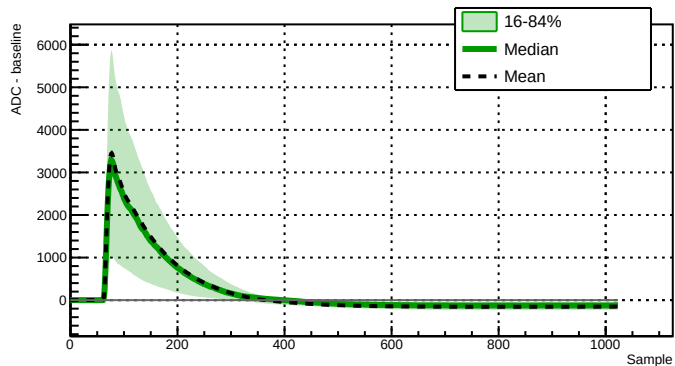
Run 039508 - Channel 2060 - 844 waveforms
