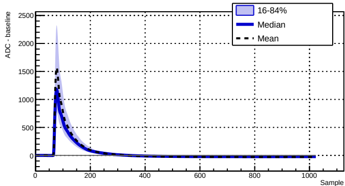
Run 039508 - Channel 2070 - 2868 waveforms
