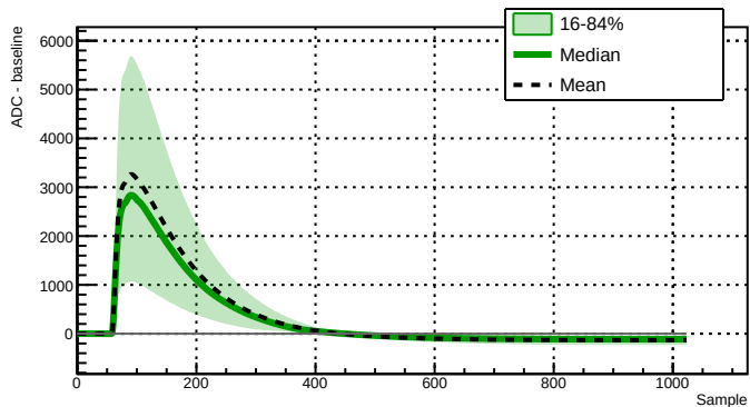
Run 039508 - Channel 2080 - 9682 waveforms
