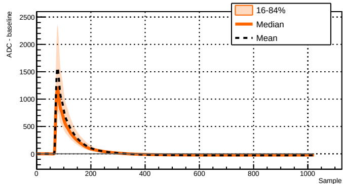
Run 039508 - Channel 2071 - 3137 waveforms
