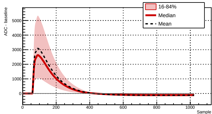
Run 039508 - Channel 2081 - 12097 waveforms
