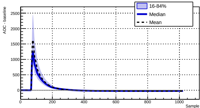
Run 039511 - Channel 2070 - 2673 waveforms
