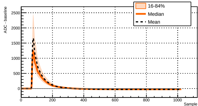
Run 039511 - Channel 2071 - 3038 waveforms
