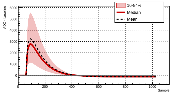
Run 039511 - Channel 2081 - 12237 waveforms
