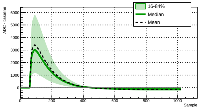
Run 039511 - Channel 2080 - 10016 waveforms
