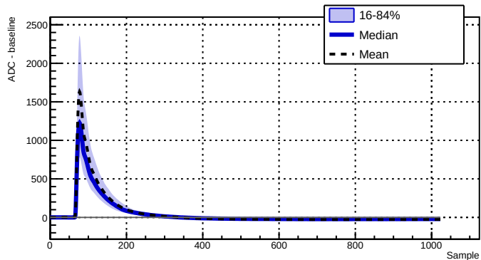
Run 039512 - Channel 2070 - 2838 waveforms
