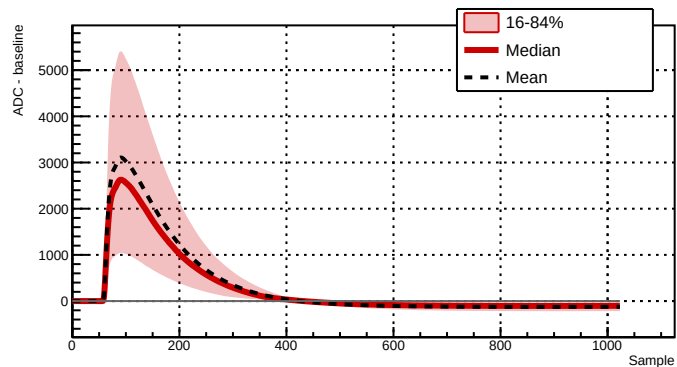
Run 039512 - Channel 2081 - 12170 waveforms
