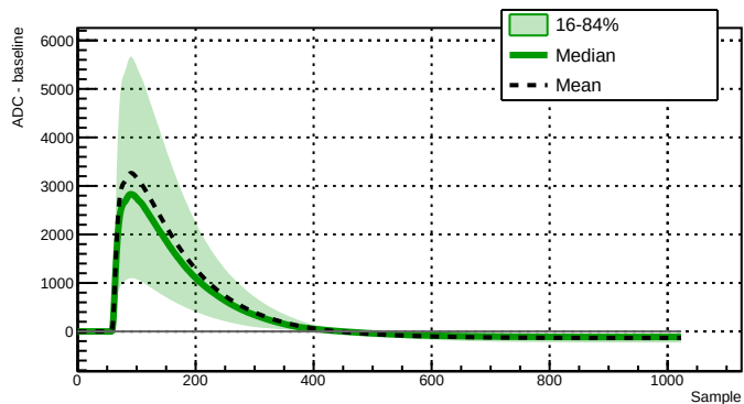
Run 039512 - Channel 2080 - 9816 waveforms
