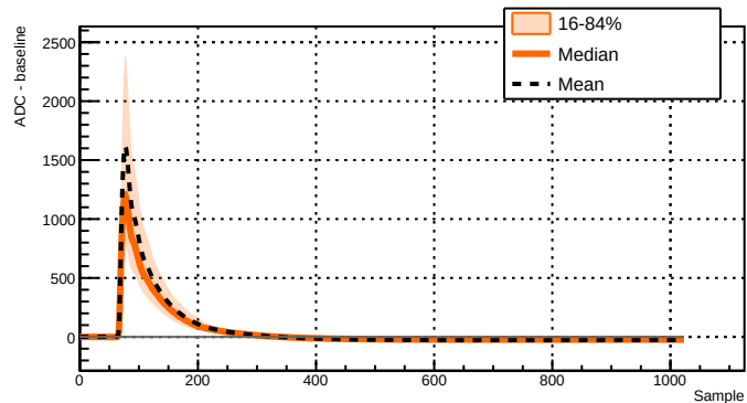
Run 039512 - Channel 2071 - 3126 waveforms
