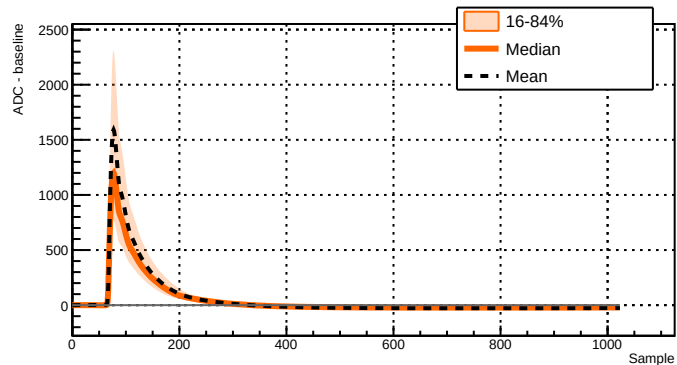
Run 039514 - Channel 2071 - 3218 waveforms
