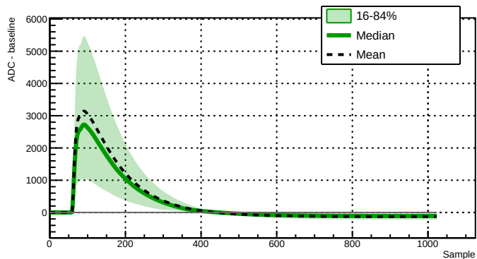
Run 039514 - Channel 2080 - 9507 waveforms
