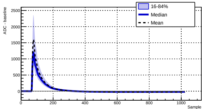
Run 039514 - Channel 2070 - 2890 waveforms
