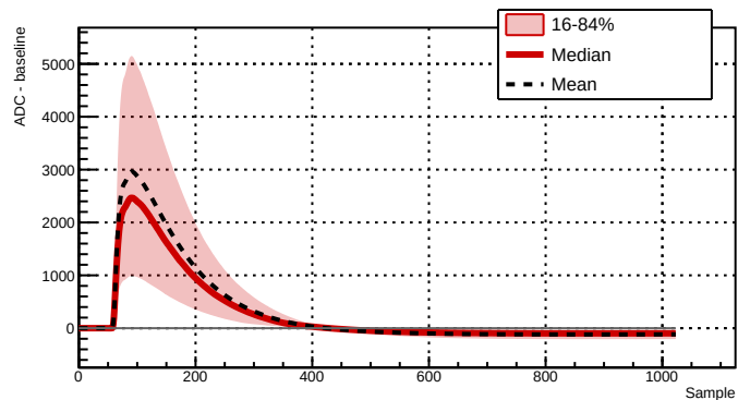
Run 039514 - Channel 2081 - 11591 waveforms
