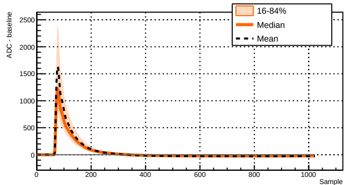
Run 039515 - Channel 2071 - 3204 waveforms
