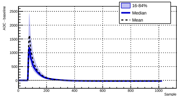
Run 039515 - Channel 2070 - 2931 waveforms
