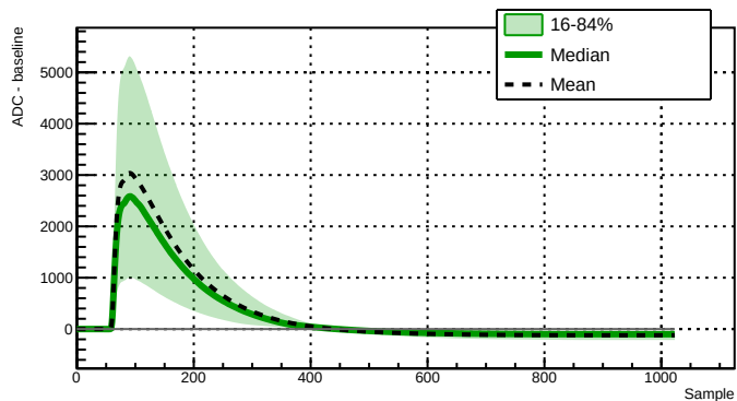
Run 039515 - Channel 2080 - 9117 waveforms
