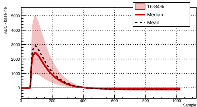
Run 039515 - Channel 2081 - 11095 waveforms
