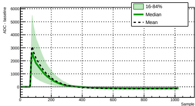
Run 039516 - Channel 2060 - 807 waveforms
