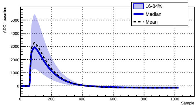
Run 039516 - Channel 2050 - 3435 waveforms
