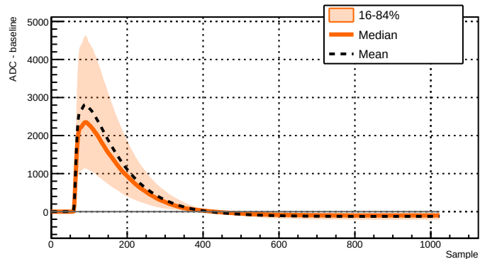
Run 039516 - Channel 2051 - 2540 waveforms
