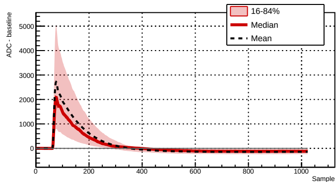
Run 039516 - Channel 2061 - 475 waveforms
