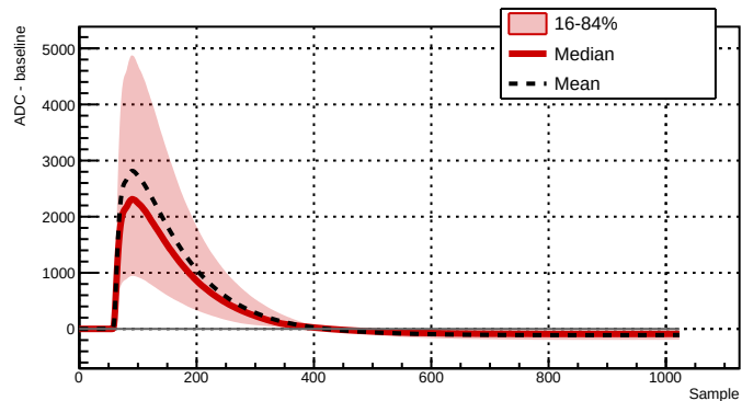
Run 039516 - Channel 2081 - 10764 waveforms
