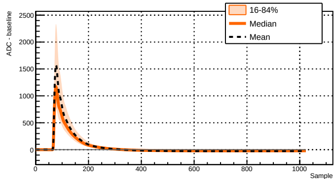
Run 039516 - Channel 2071 - 3119 waveforms
