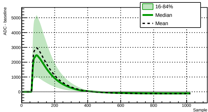
Run 039516 - Channel 2080 - 8775 waveforms
