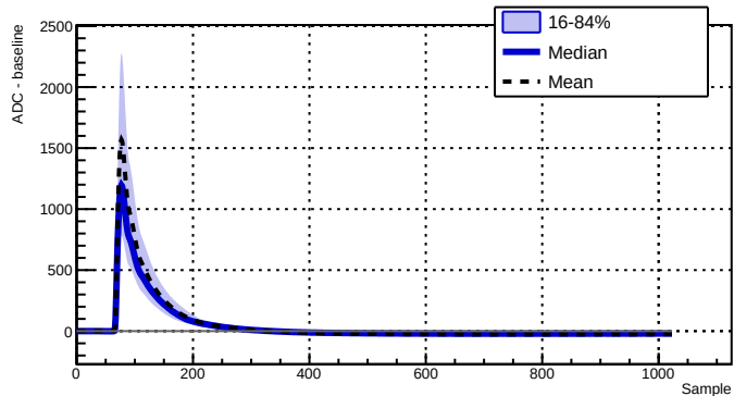
Run 039516 - Channel 2070 - 2871 waveforms
