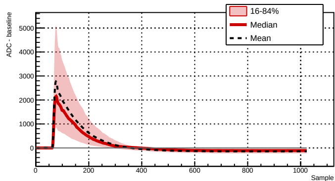
Run 039518 - Channel 2061 - 460 waveforms
