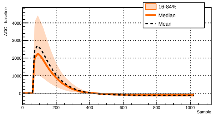
Run 039518 - Channel 2051 - 2371 waveforms
