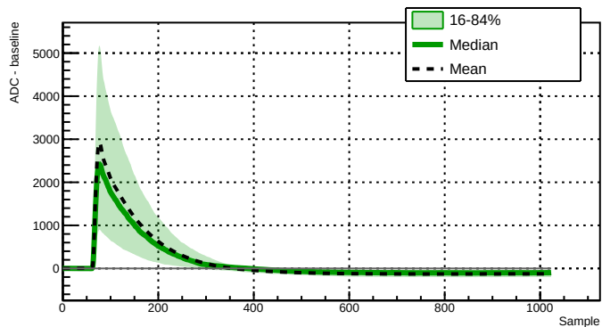
Run 039518 - Channel 2060 - 734 waveforms
