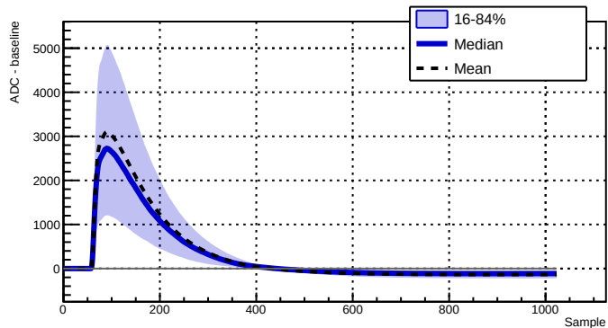
Run 039518 - Channel 2050 - 3069 waveforms
