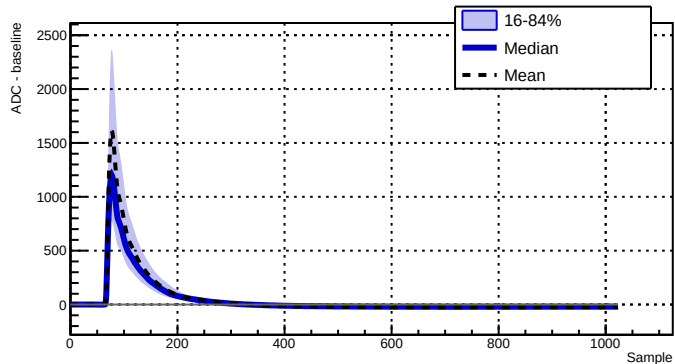
Run 039518 - Channel 2070 - 2951 waveforms
