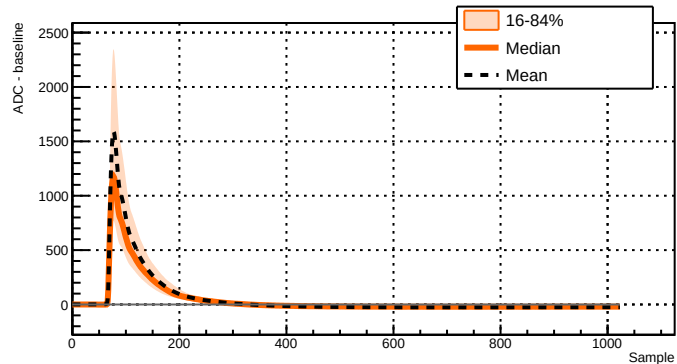
Run 039518 - Channel 2071 - 3222 waveforms
