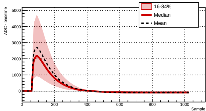
Run 039518 - Channel 2081 - 10543 waveforms
