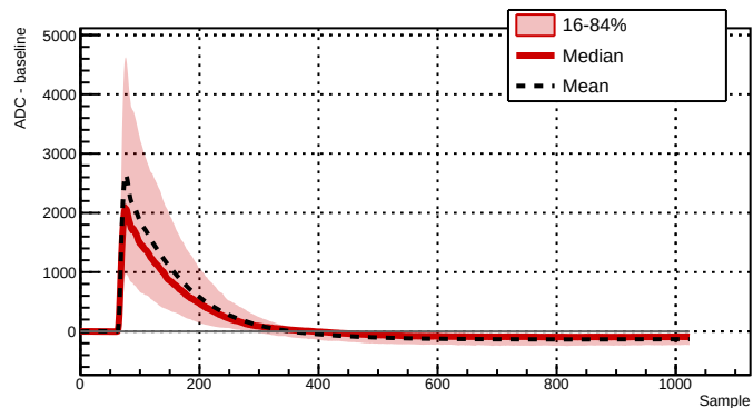
Run 039519 - Channel 2061 - 475 waveforms
