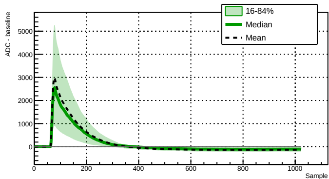
Run 039519 - Channel 2060 - 740 waveforms
