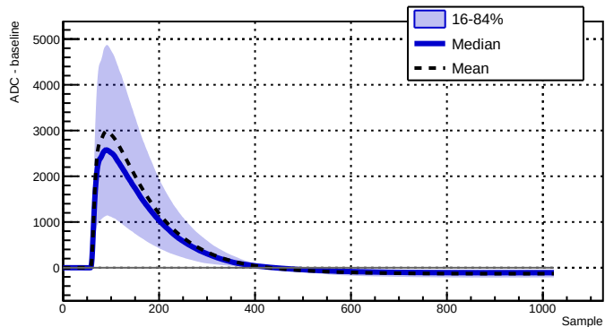
Run 039519 - Channel 2050 - 2992 waveforms
