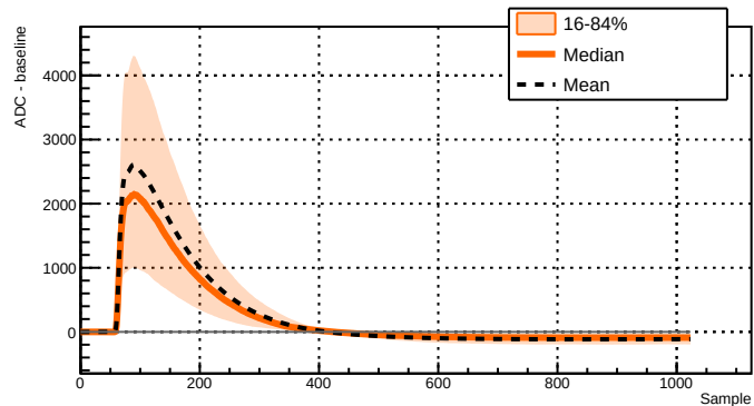
Run 039519 - Channel 2051 - 2313 waveforms
