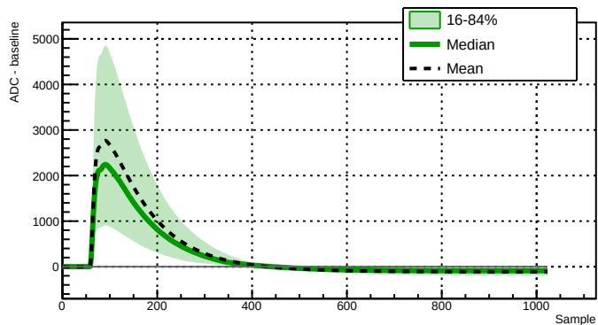
Run 039519 - Channel 2080 - 8364 waveforms
