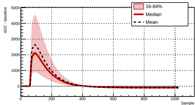
Run 039519 - Channel 2081 - 10222 waveforms
