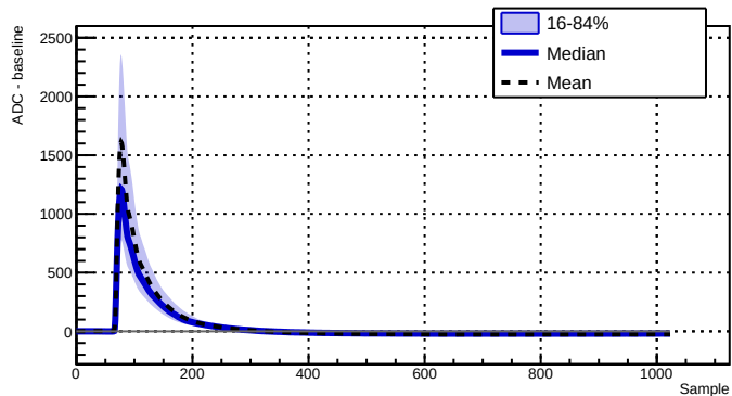
Run 039519 - Channel 2070 - 2965 waveforms
