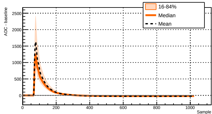
Run 039519 - Channel 2071 - 3205 waveforms
