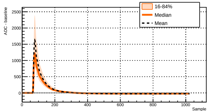
Run 039521 - Channel 2071 - 3037 waveforms
