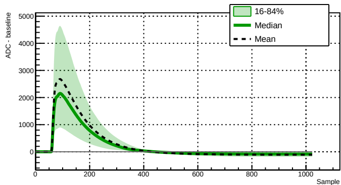
Run 039521 - Channel 2080 - 8013 waveforms
