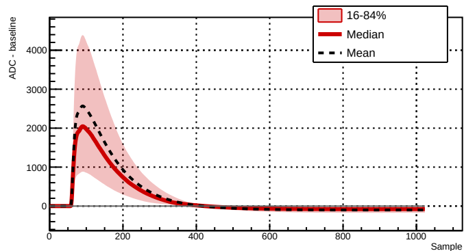
Run 039521 - Channel 2081 - 9962 waveforms
