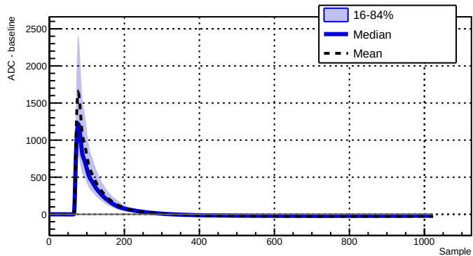
Run 039521 - Channel 2070 - 2880 waveforms
