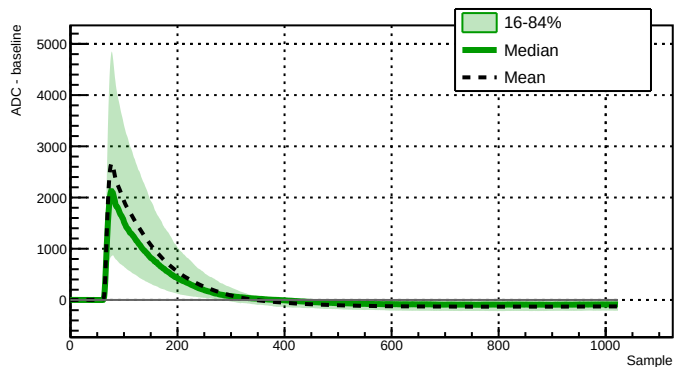
Run 039522 - Channel 2060 - 642 waveforms
