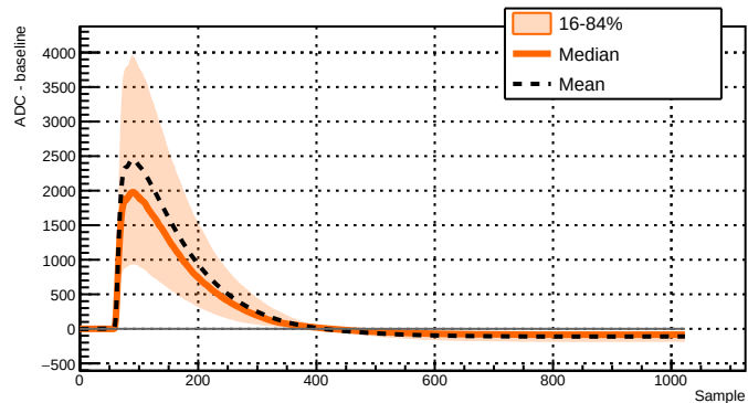
Run 039522 - Channel 2051 - 2057 waveforms
