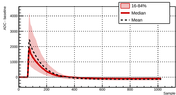
Run 039522 - Channel 2061 - 404 waveforms
