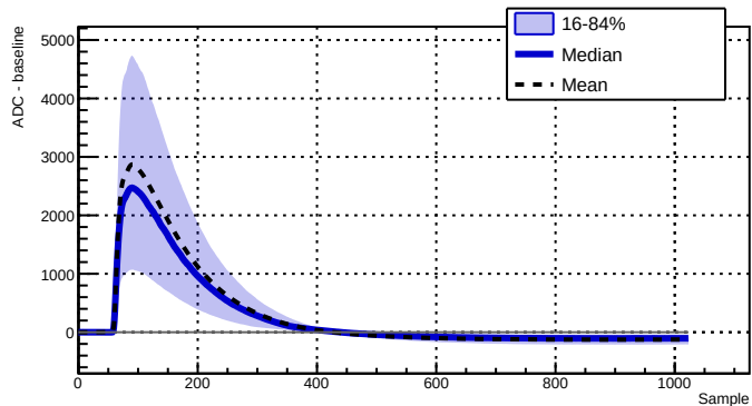
Run 039522 - Channel 2050 - 2706 waveforms
