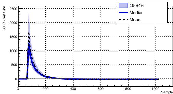
Run 039522 - Channel 2070 - 2902 waveforms
