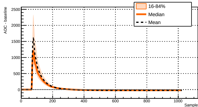
Run 039522 - Channel 2071 - 3123 waveforms
