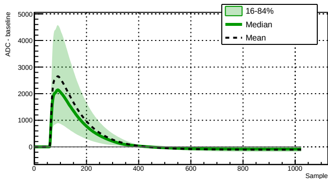
Run 039522 - Channel 2080 - 7866 waveforms
