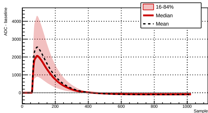
Run 039522 - Channel 2081 - 9776 waveforms
