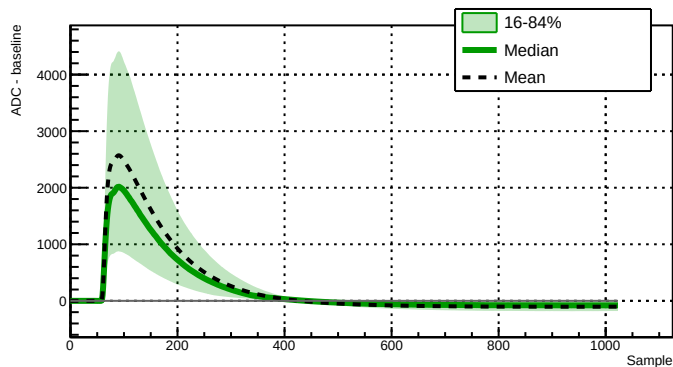
Run 039523 - Channel 2080 - 7640 waveforms
