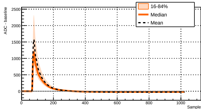
Run 039523 - Channel 2071 - 2990 waveforms
