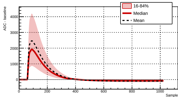
Run 039523 - Channel 2081 - 9424 waveforms
