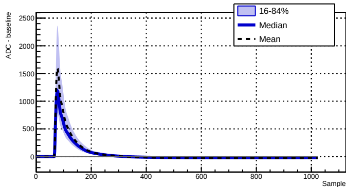
Run 039523 - Channel 2070 - 2803 waveforms
