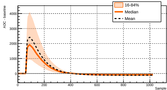
Run 039525 - Channel 2051 - 1908 waveforms
