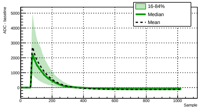
Run 039525 - Channel 2060 - 647 waveforms
