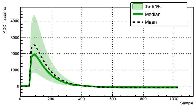
Run 039526 - Channel 2080 - 7304 waveforms
