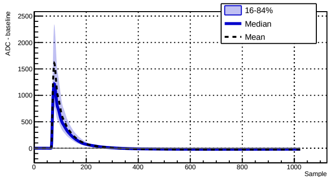
Run 039526 - Channel 2070 - 2863 waveforms
