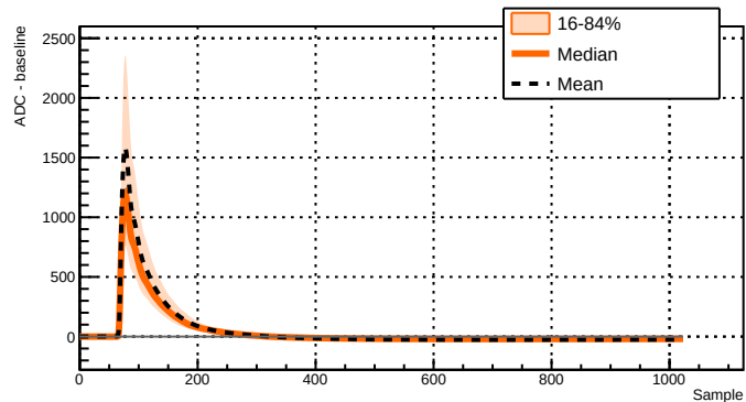
Run 039526 - Channel 2071 - 3066 waveforms
