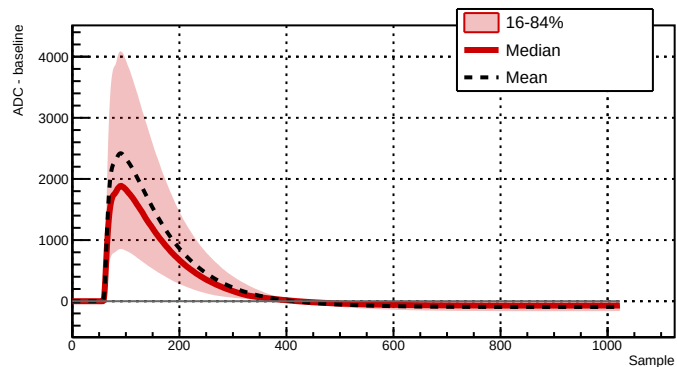
Run 039526 - Channel 2081 - 9111 waveforms
