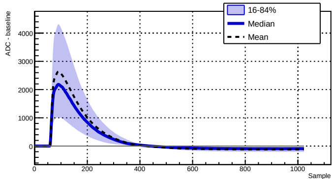
Run 039527 - Channel 2050 - 2543 waveforms
