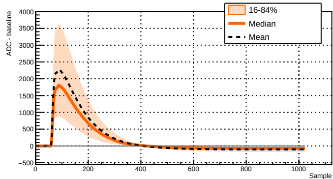
Run 039527 - Channel 2051 - 1848 waveforms
