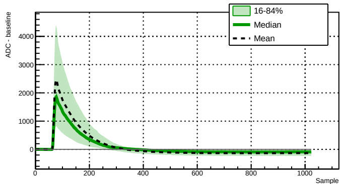
Run 039527 - Channel 2060 - 621 waveforms
