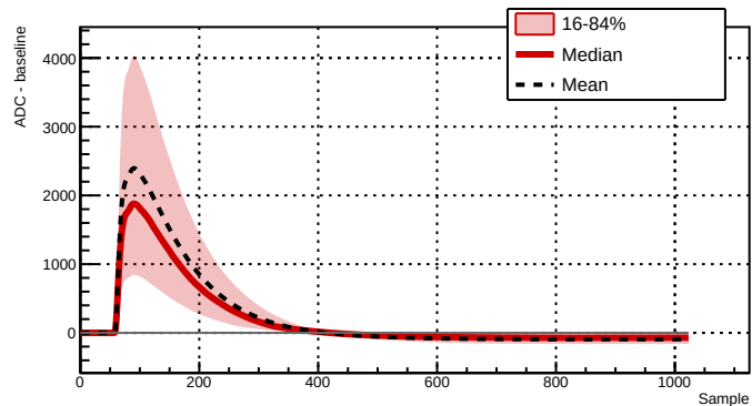
Run 039527 - Channel 2081 - 8947 waveforms
