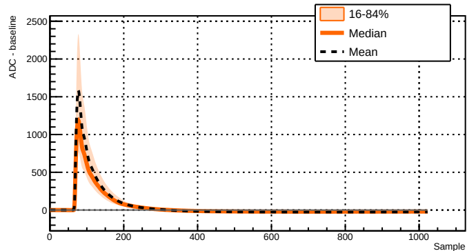
Run 039527 - Channel 2071 - 2959 waveforms
