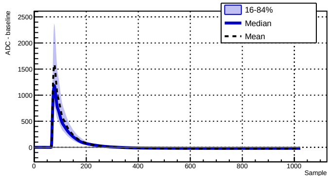
Run 039527 - Channel 2070 - 2771 waveforms
