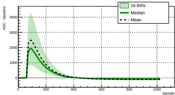
Run 039527 - Channel 2080 - 7271 waveforms
