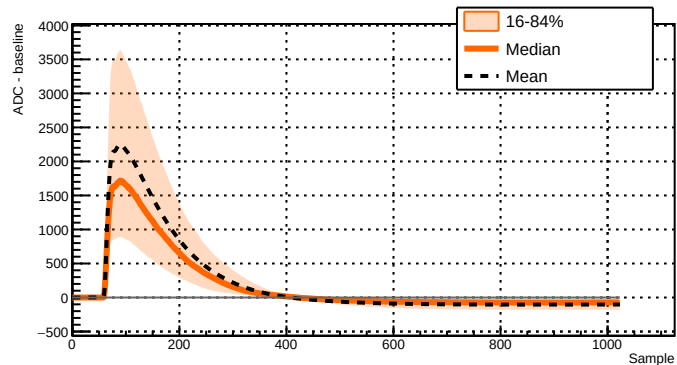
Run 039528 - Channel 2051 - 1714 waveforms
