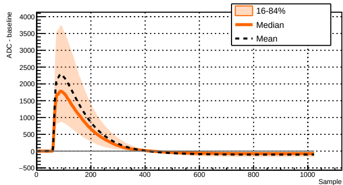
Run 039529 - Channel 2051 - 1660 waveforms
