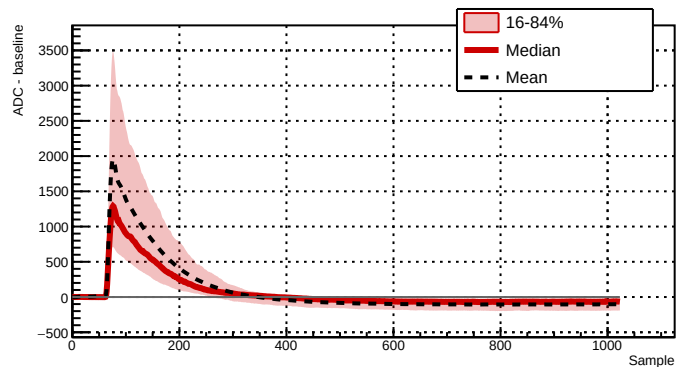
Run 039529 - Channel 2061 - 338 waveforms
