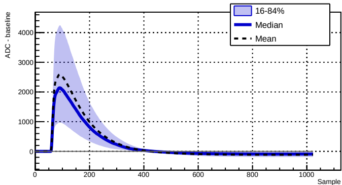
Run 039529 - Channel 2050 - 2301 waveforms
