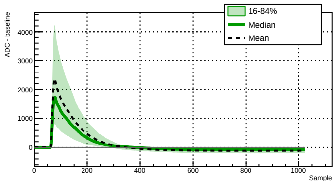
Run 039529 - Channel 2060 - 594 waveforms
