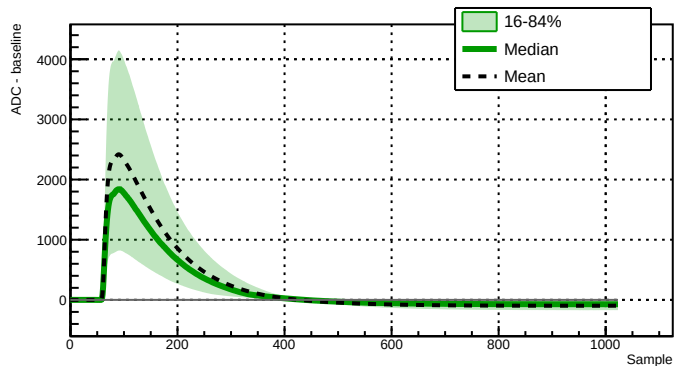
Run 039529 - Channel 2080 - 6912 waveforms
