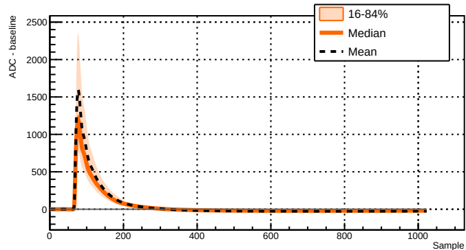
Run 039529 - Channel 2071 - 2920 waveforms
