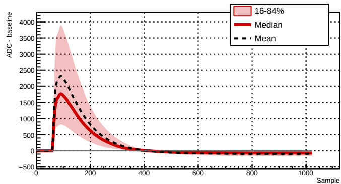
Run 039529 - Channel 2081 - 8555 waveforms
