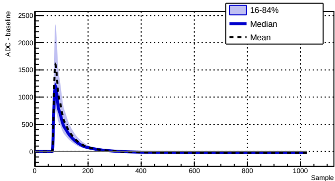
Run 039529 - Channel 2070 - 2736 waveforms
