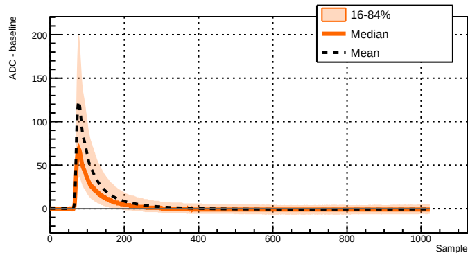
Run 039787 - Channel 2071 - 40286 waveforms
