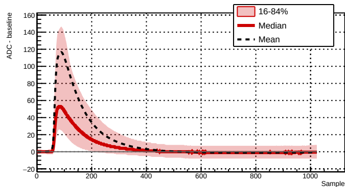
Run 039787 - Channel 2081 - 25411 waveforms
