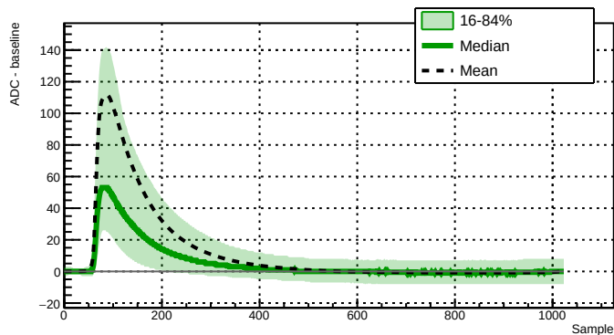
Run 039787 - Channel 2080 - 24771 waveforms
