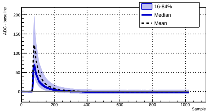
Run 039787 - Channel 2070 - 40614 waveforms
